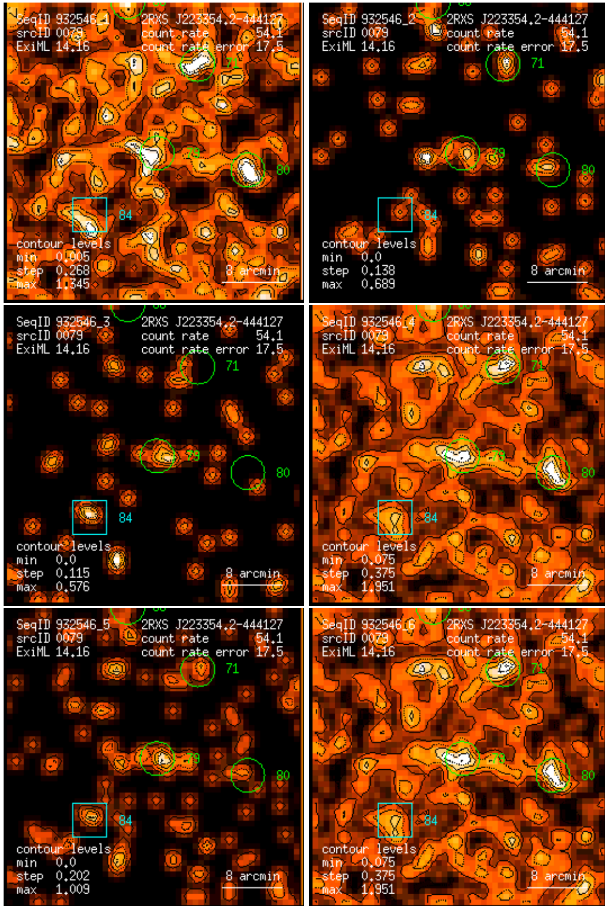
Figure 79: RASS 932546: detection 0079: band rate images, Gaussian filter: (1) PSPC channels 11 – 41, (2) 52 – 90, (3) 91 – 201, (4) 11 – 235, (5) 52 – 201, (6) 11 – 201. Broad band rates in counts/ks. Band rate contour levels in counts/ks/arcmin 2 .
