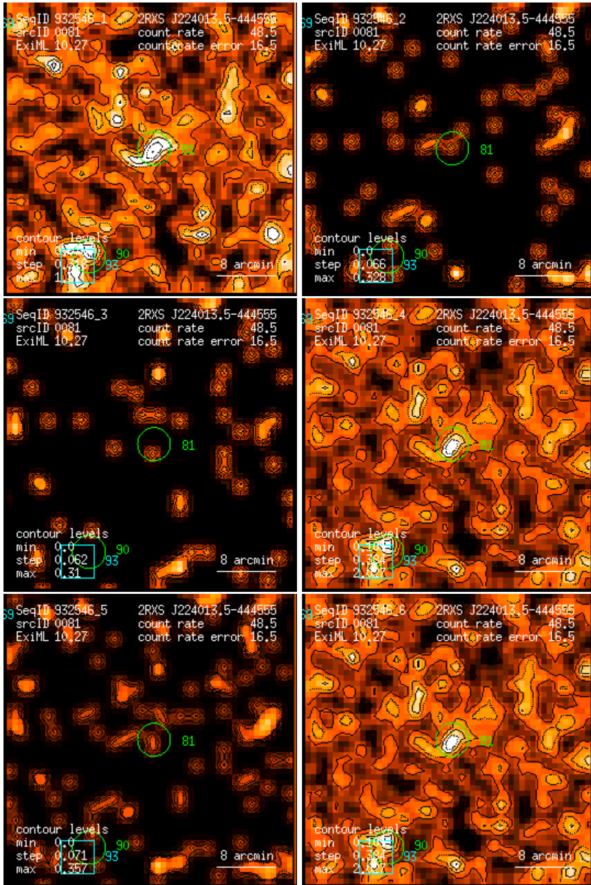
Figure 81: RASS 932546: detection 0081: band rate images, Gaussian filter: (1) PSPC channels 11 – 41, (2) 52 – 90, (3) 91 – 201, (4) 11 – 235, (5) 52 – 201, (6) 11 – 201. Broad band rates in counts/ks. Band rate contour levels in counts/ks/arcmin 2 .
