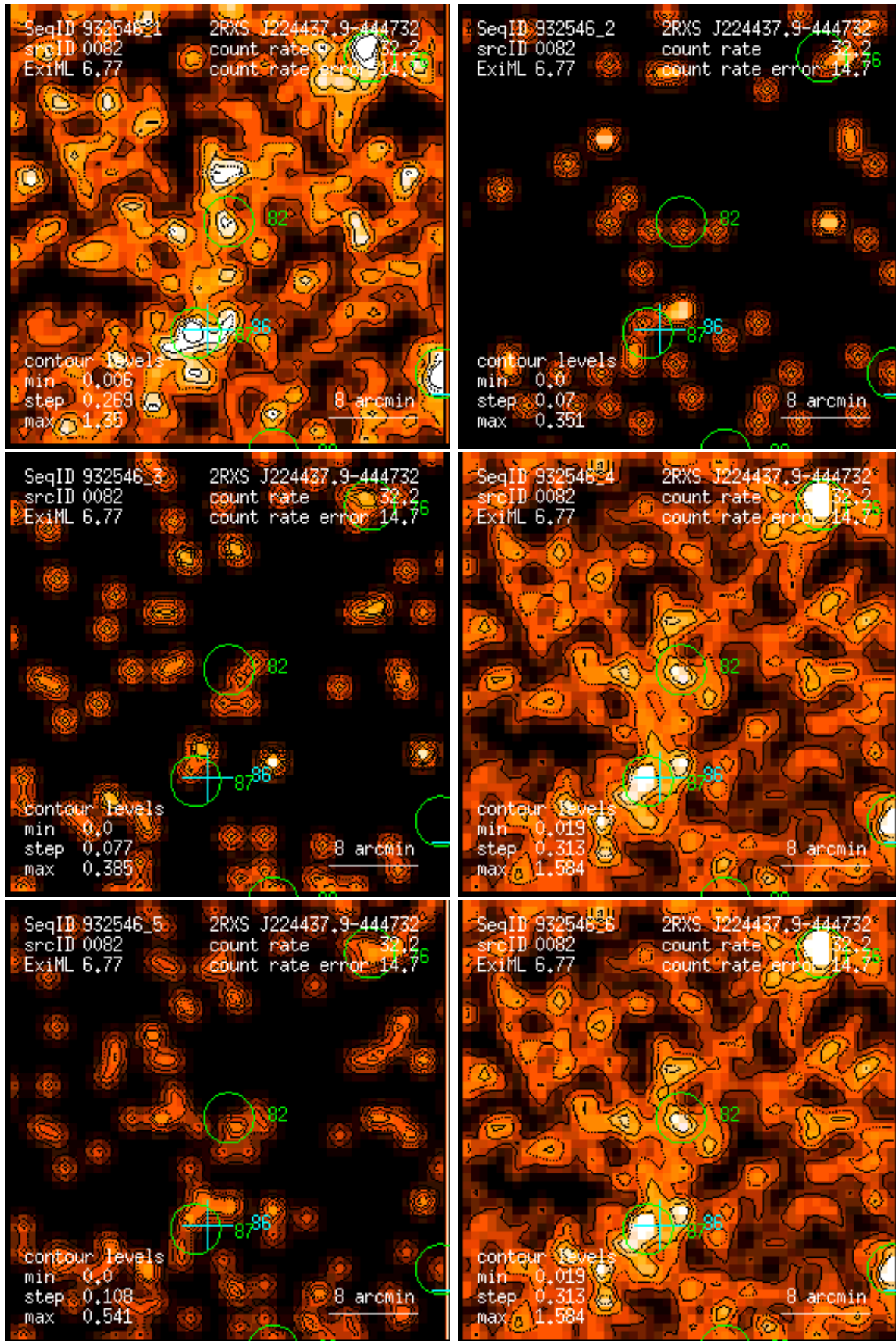
Figure 82: RASS 932546: detection 0082: band rate images, Gaussian filter: (1) PSPC channels 11 – 41, (2) 52 – 90, (3) 91 – 201, (4) 11 – 235, (5) 52 – 201, (6) 11 – 201. Broad band rates in counts/ks. Band rate contour levels in counts/ks/arcmin 2 .
