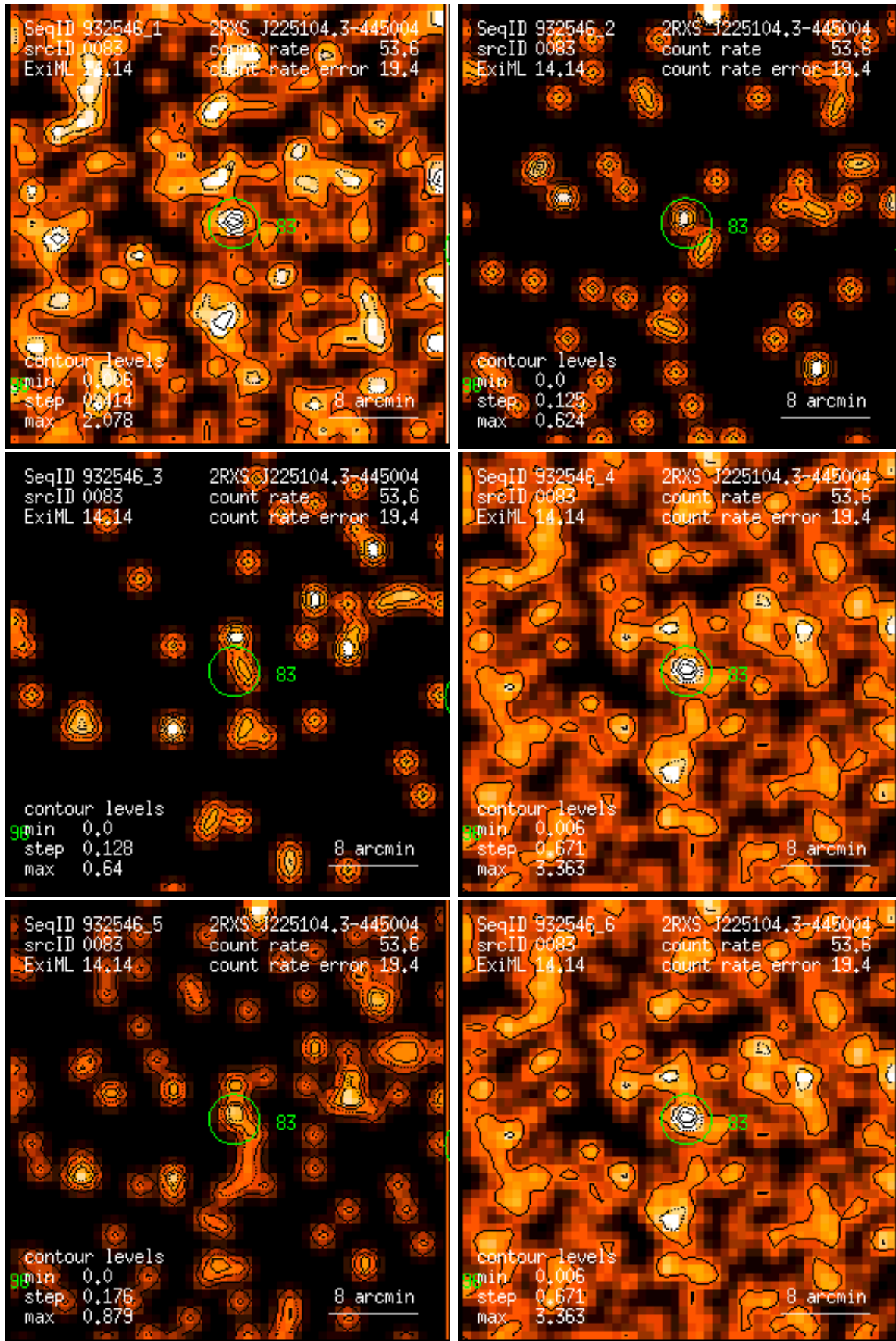
Figure 83: RASS 932546: detection 0083: band rate images, Gaussian filter: (1) PSPC channels 11 – 41, (2) 52 – 90, (3) 91 – 201, (4) 11 – 235, (5) 52 – 201, (6) 11 – 201. Broad band rates in counts/ks. Band rate contour levels in counts/ks/arcmin 2 .
