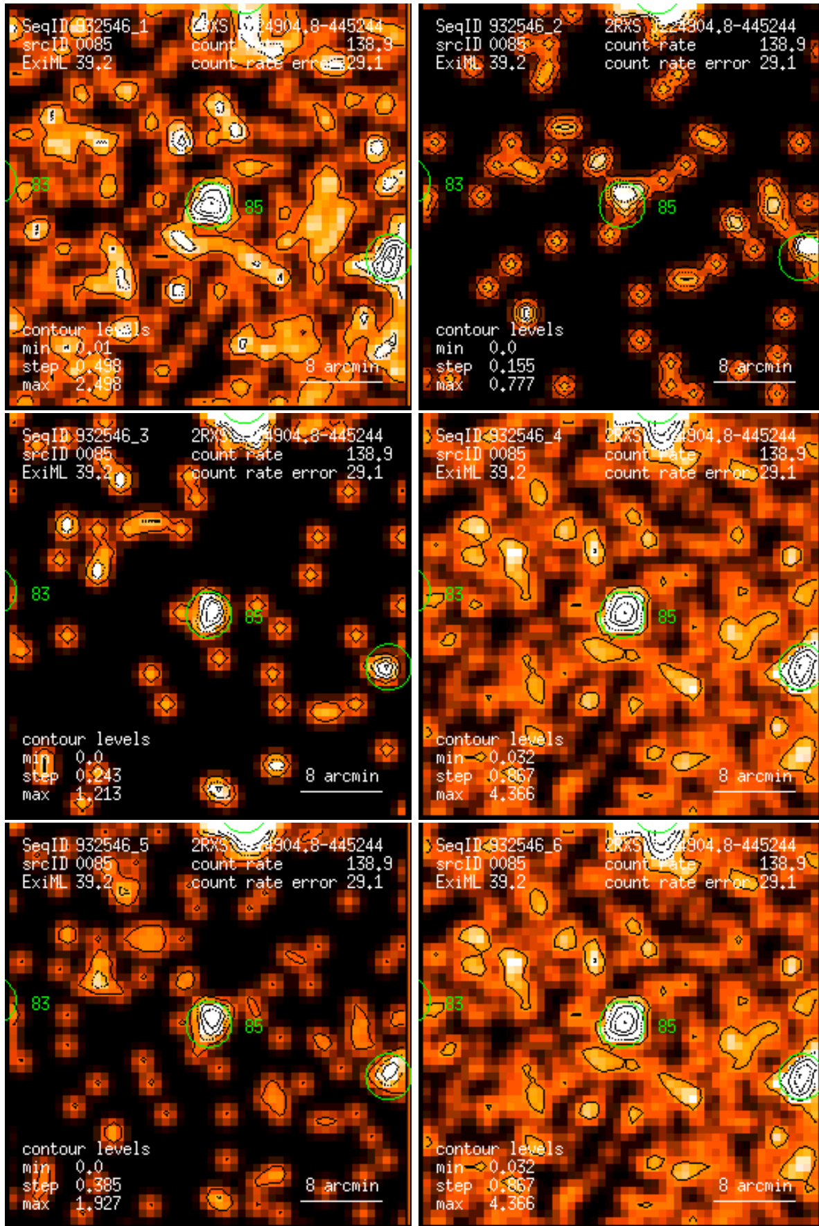
Figure 85: RASS 932546: detection 0085: band rate images, Gaussian filter: (1) PSPC channels 11 – 41, (2) 52 – 90, (3) 91 – 201, (4) 11 – 235, (5) 52 – 201, (6) 11 – 201. Broad band rates in counts/ks. Band rate contour levels in counts/ks/arcmin 2 .
