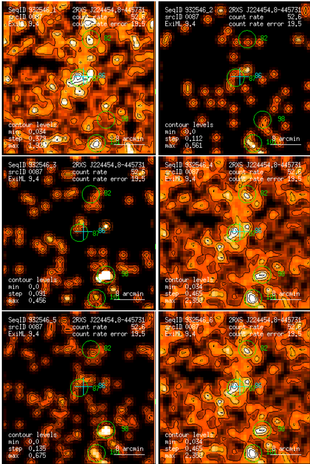
Figure 87: RASS 932546: detection 0087: band rate images, Gaussian filter: (1) PSPC channels 11 – 41, (2) 52 – 90, (3) 91 – 201, (4) 11 – 235, (5) 52 – 201, (6) 11 – 201. Broad band rates in counts/ks. Band rate contour levels in counts/ks/arcmin 2 .
