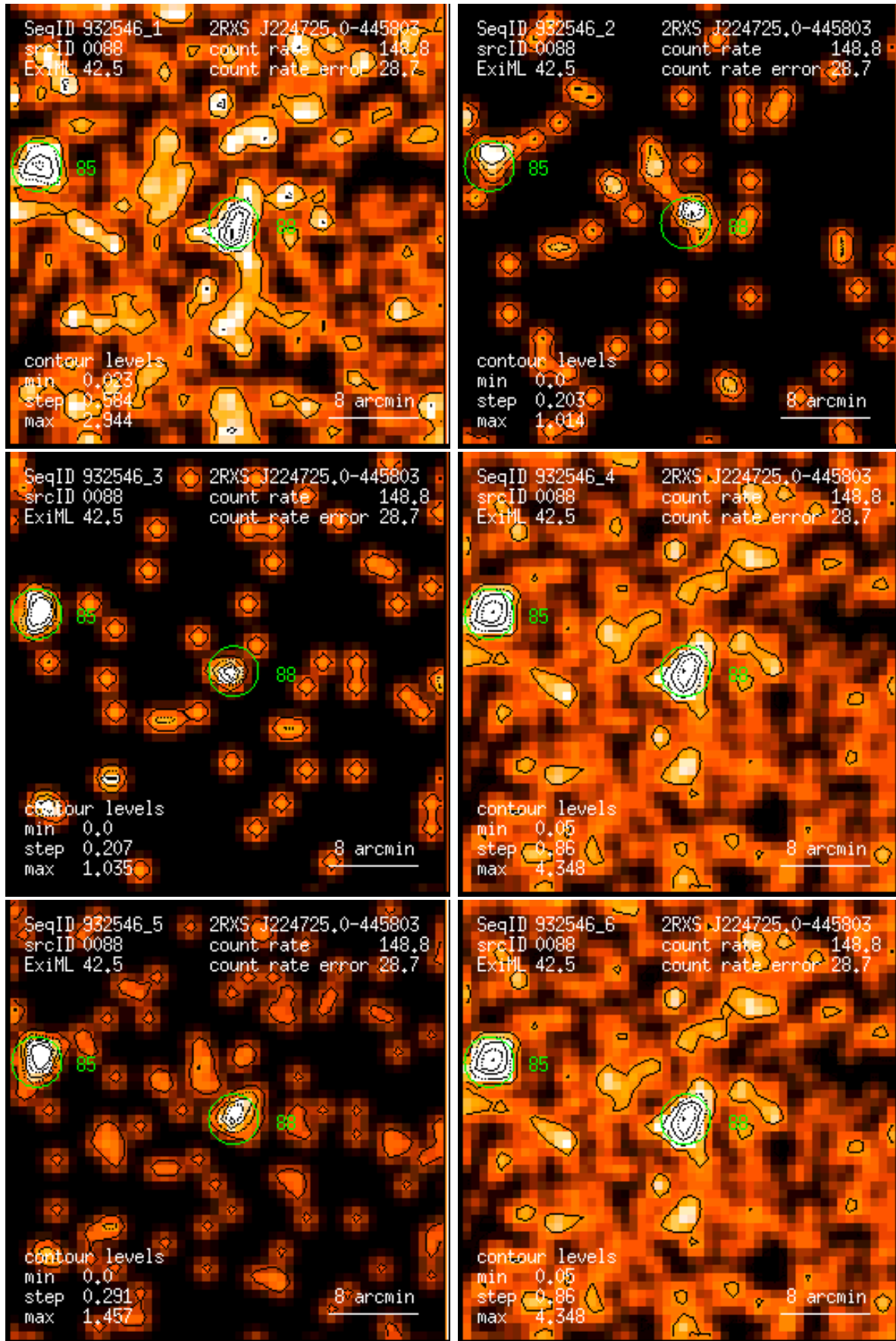
Figure 88: RASS 932546: detection 0088: band rate images, Gaussian filter: (1) PSPC channels 11 – 41, (2) 52 – 90, (3) 91 – 201, (4) 11 – 235, (5) 52 – 201, (6) 11 – 201. Broad band rates in counts/ks. Band rate contour levels in counts/ks/arcmin 2 .
