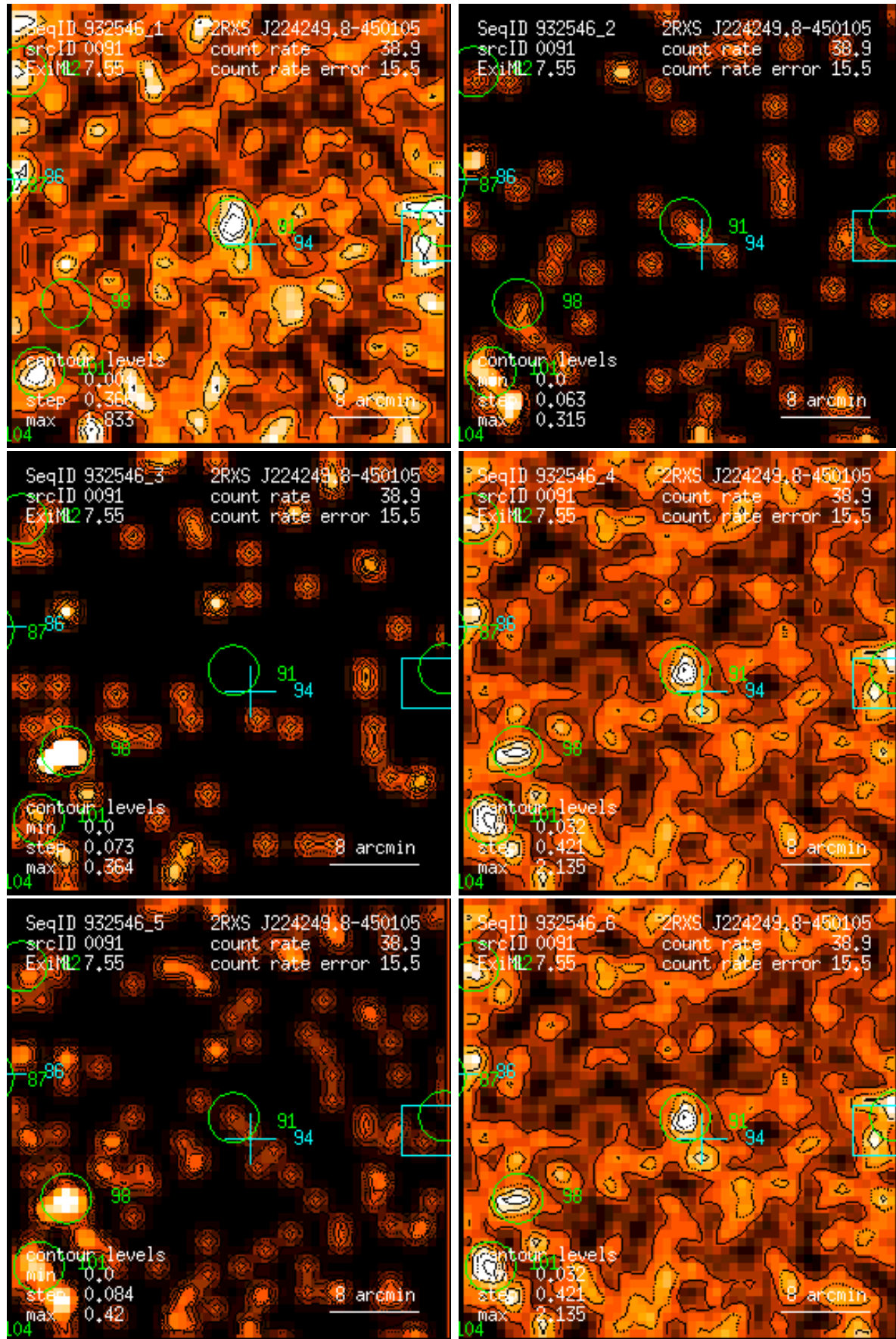
Figure 91: RASS 932546: detection 0091: band rate images, Gaussian filter: (1) PSPC channels 11 – 41, (2) 52 – 90, (3) 91 – 201, (4) 11 – 235, (5) 52 – 201, (6) 11 – 201. Broad band rates in counts/ks. Band rate contour levels in counts/ks/arcmin 2 .
