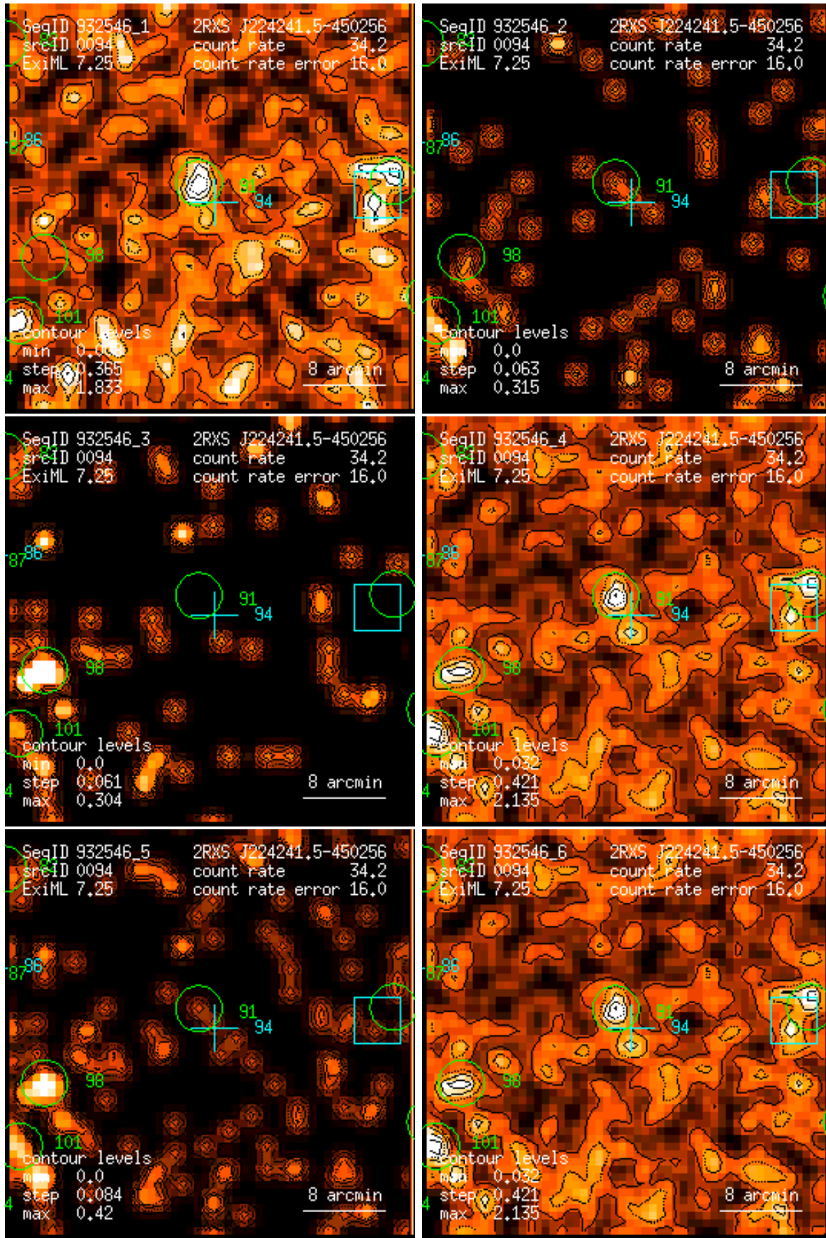
Figure 94: RASS 932546: detection 0094: band rate images, Gaussian filter: (1) PSPC channels 11 – 41, (2) 52 – 90, (3) 91 – 201, (4) 11 – 235, (5) 52 – 201, (6) 11 – 201. Broad band rates in counts/ks. Band rate contour levels in counts/ks/arcmin 2 .
