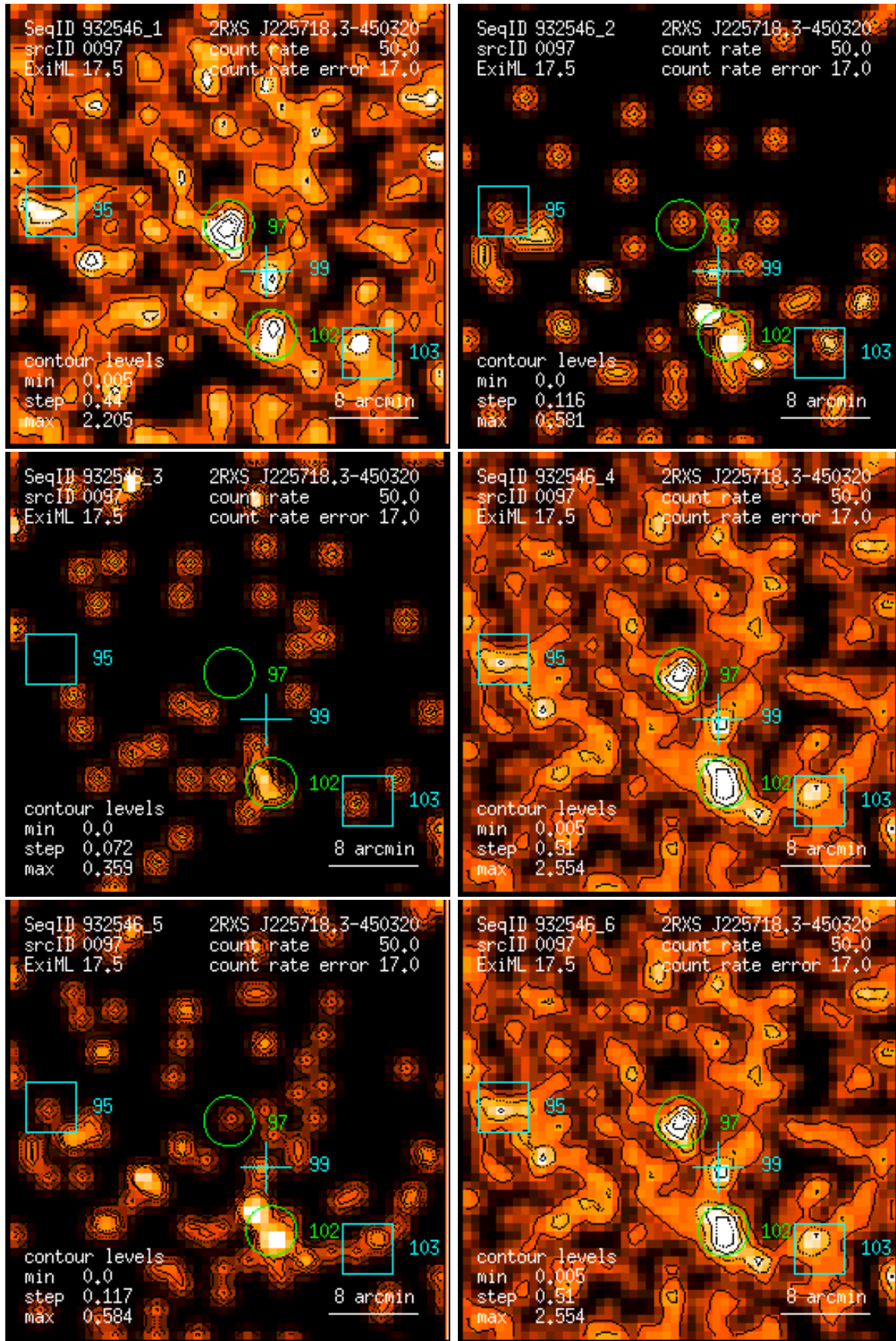
Figure 97: RASS 932546: detection 0097: band rate images, Gaussian filter: (1) PSPC channels 11 – 41, (2) 52 – 90, (3) 91 – 201, (4) 11 – 235, (5) 52 – 201, (6) 11 – 201. Broad band rates in counts/ks. Band rate contour levels in counts/ks/arcmin 2 .
