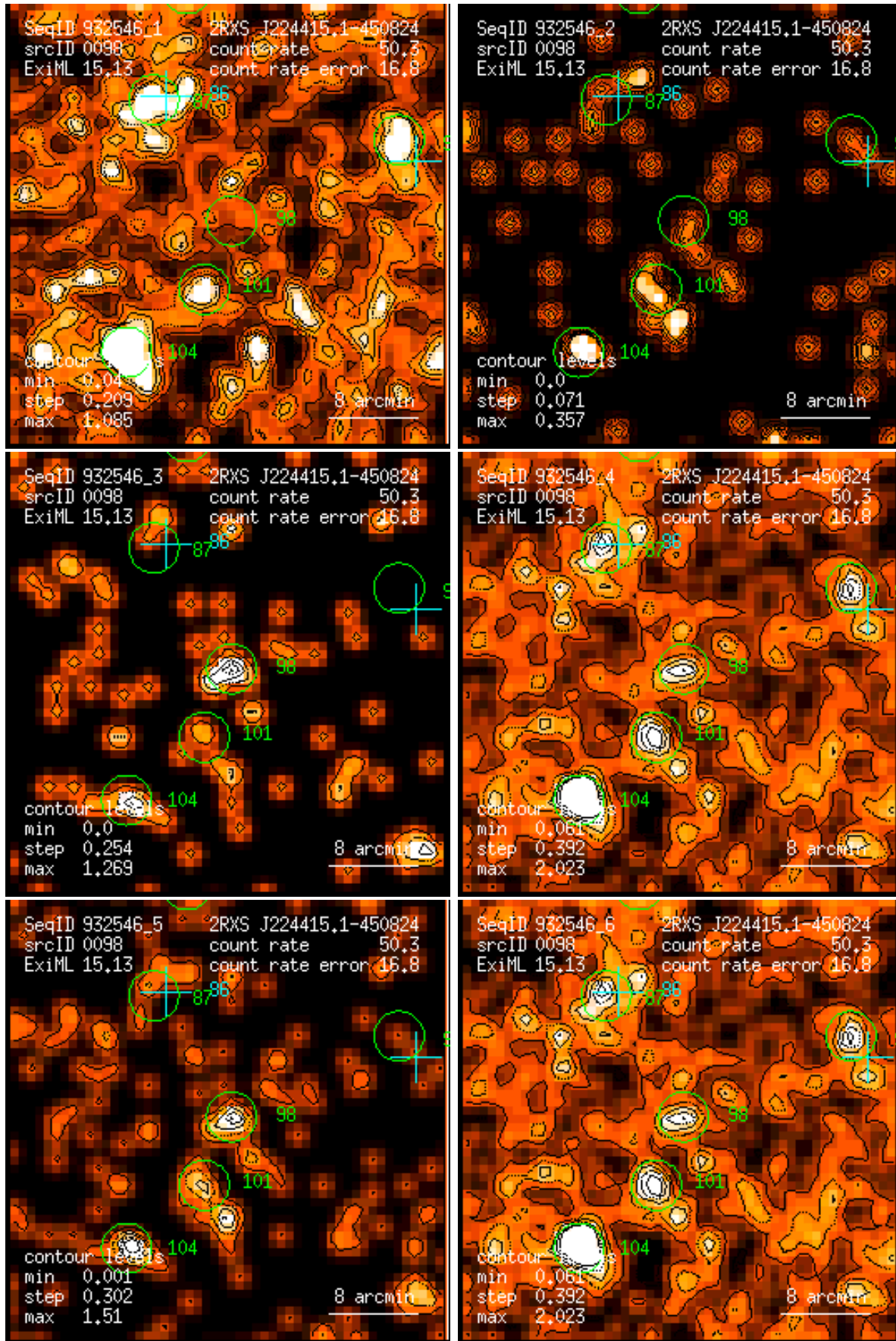
Figure 98: RASS 932546: detection 0098: band rate images, Gaussian filter: (1) PSPC channels 11 – 41, (2) 52 – 90, (3) 91 – 201, (4) 11 – 235, (5) 52 – 201, (6) 11 – 201. Broad band rates in counts/ks. Band rate contour levels in counts/ks/arcmin 2 .
