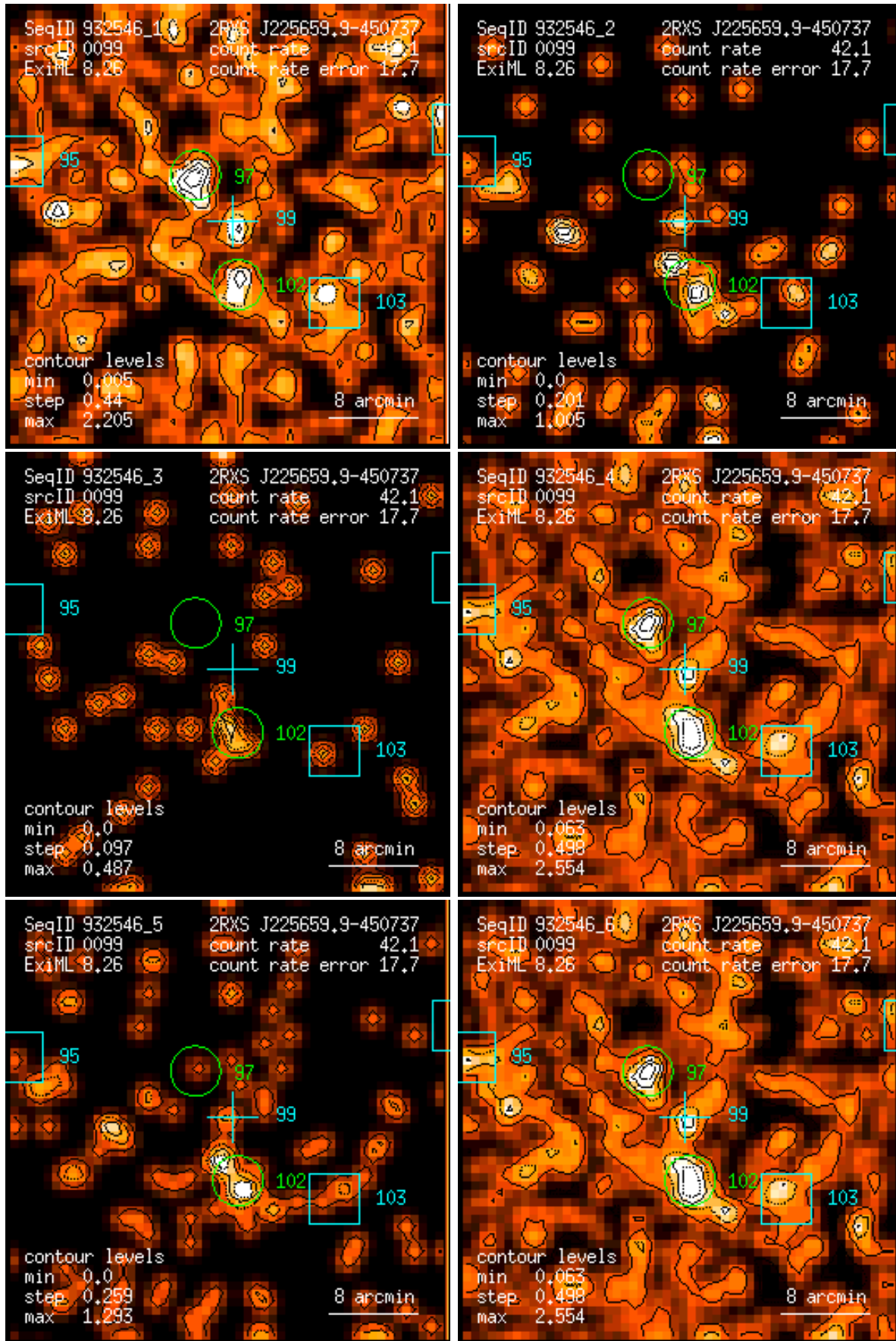
Figure 99: RASS 932546: detection 0099: band rate images, Gaussian filter: (1) PSPC channels 11 – 41, (2) 52 – 90, (3) 91 – 201, (4) 11 – 235, (5) 52 – 201, (6) 11 – 201. Broad band rates in counts/ks. Band rate contour levels in counts/ks/arcmin 2 .
