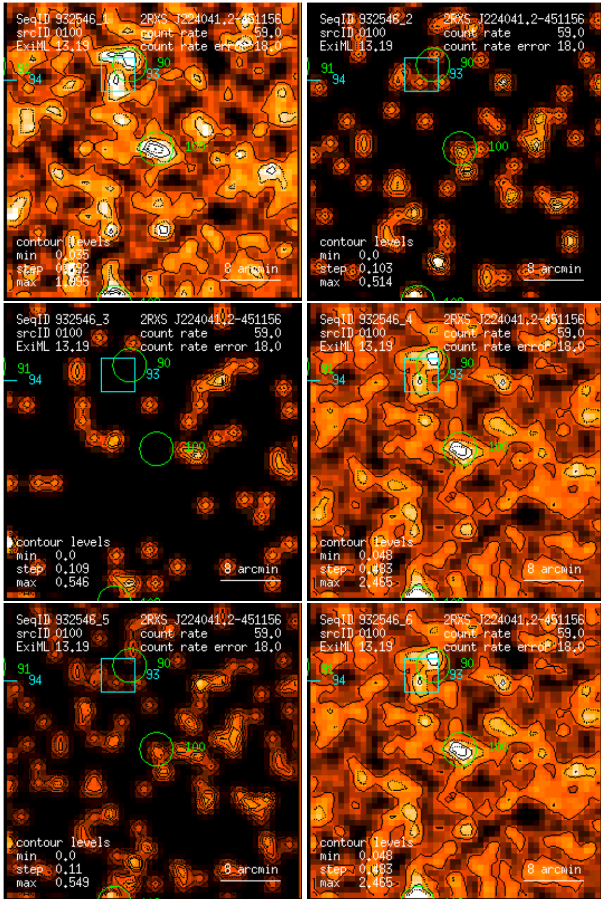
Figure 100: RASS 932546: detection 0100: band rate images, Gaussian filter: (1) PSPC channels 11 – 41, (2) 52 – 90, (3) 91 – 201, (4) 11 – 235, (5) 52 – 201, (6) 11 – 201. Broad band rates in counts/ks. Band rate contour levels in counts/ks/arcmin 2 .
