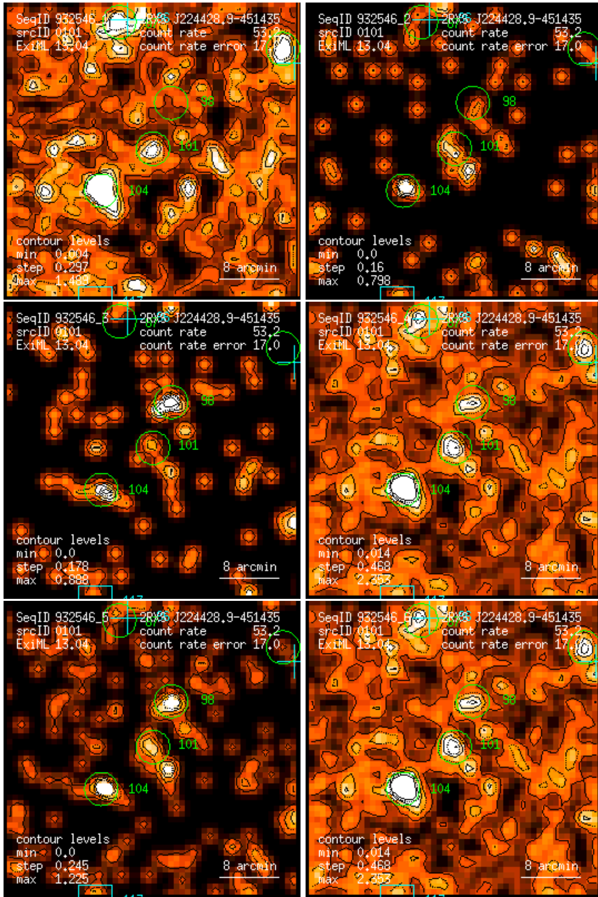
Figure 101: RASS 932546: detection 0101: band rate images, Gaussian filter: (1) PSPC channels 11 – 41, (2) 52 – 90, (3) 91 – 201, (4) 11 – 235, (5) 52 – 201, (6) 11 – 201. Broad band rates in counts/ks. Band rate contour levels in counts/ks/arcmin 2 .
