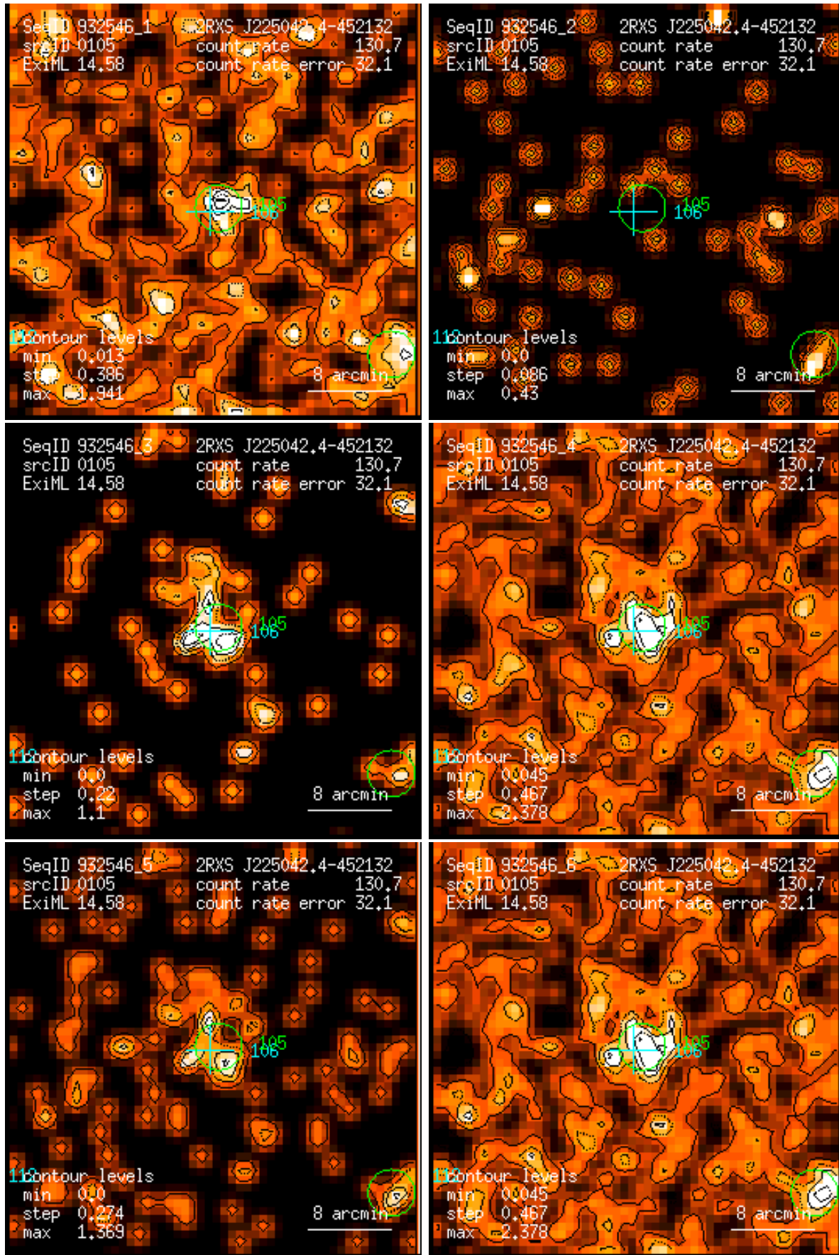
Figure 105: RASS 932546: detection 0105: band rate images, Gaussian filter: (1) PSPC channels 11 – 41, (2) 52 – 90, (3) 91 – 201, (4) 11 – 235, (5) 52 – 201, (6) 11 – 201. Broad band rates in counts/ks. Band rate contour levels in counts/ks/arcmin 2 .
