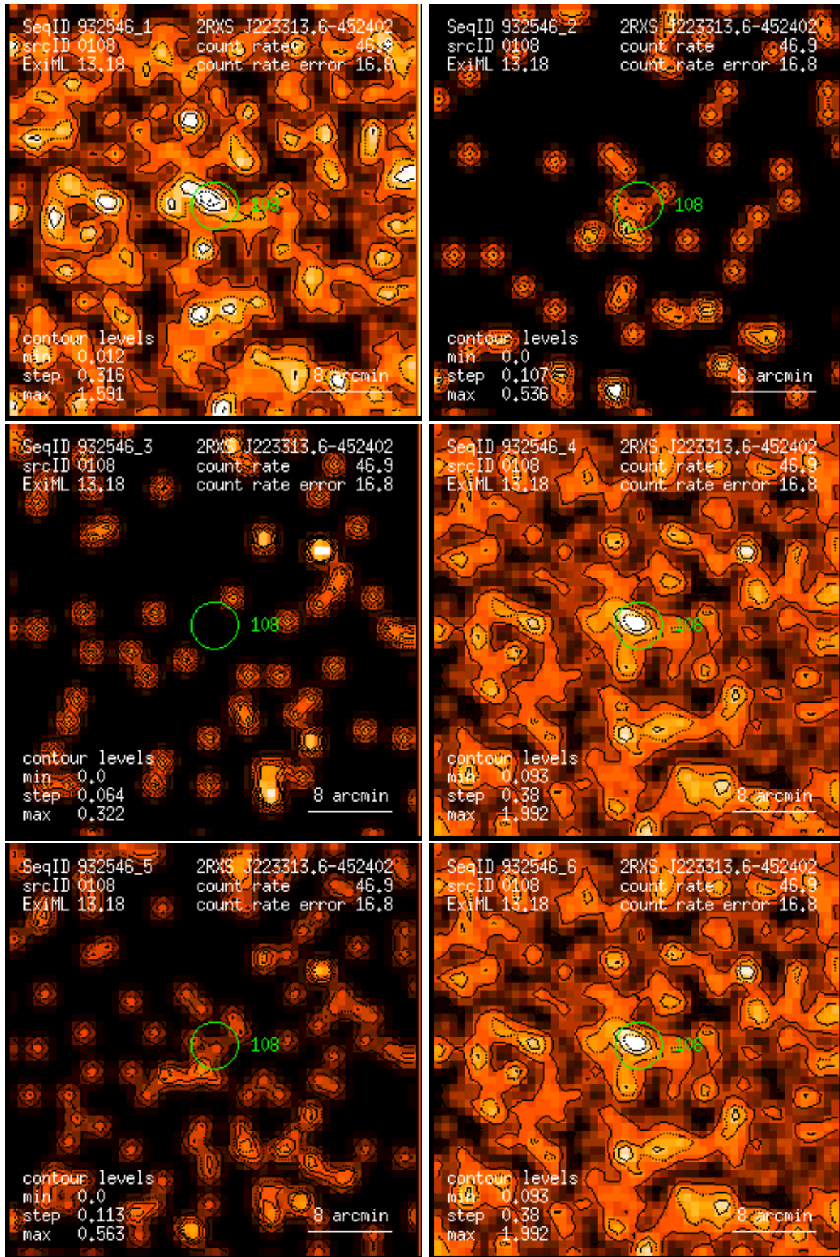
Figure 108: RASS 932546: detection 0108: band rate images, Gaussian filter: (1) PSPC channels 11 – 41, (2) 52 – 90, (3) 91 – 201, (4) 11 – 235, (5) 52 – 201, (6) 11 – 201. Broad band rates in counts/ks. Band rate contour levels in counts/ks/arcmin 2 .
