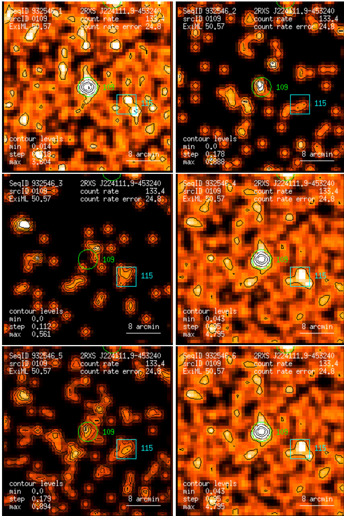
Figure 109: RASS 932546: detection 0109: band rate images, Gaussian filter: (1) PSPC channels 11 – 41, (2) 52 – 90, (3) 91 – 201, (4) 11 – 235, (5) 52 – 201, (6) 11 – 201. Broad band rates in counts/ks. Band rate contour levels in counts/ks/arcmin 2 .
