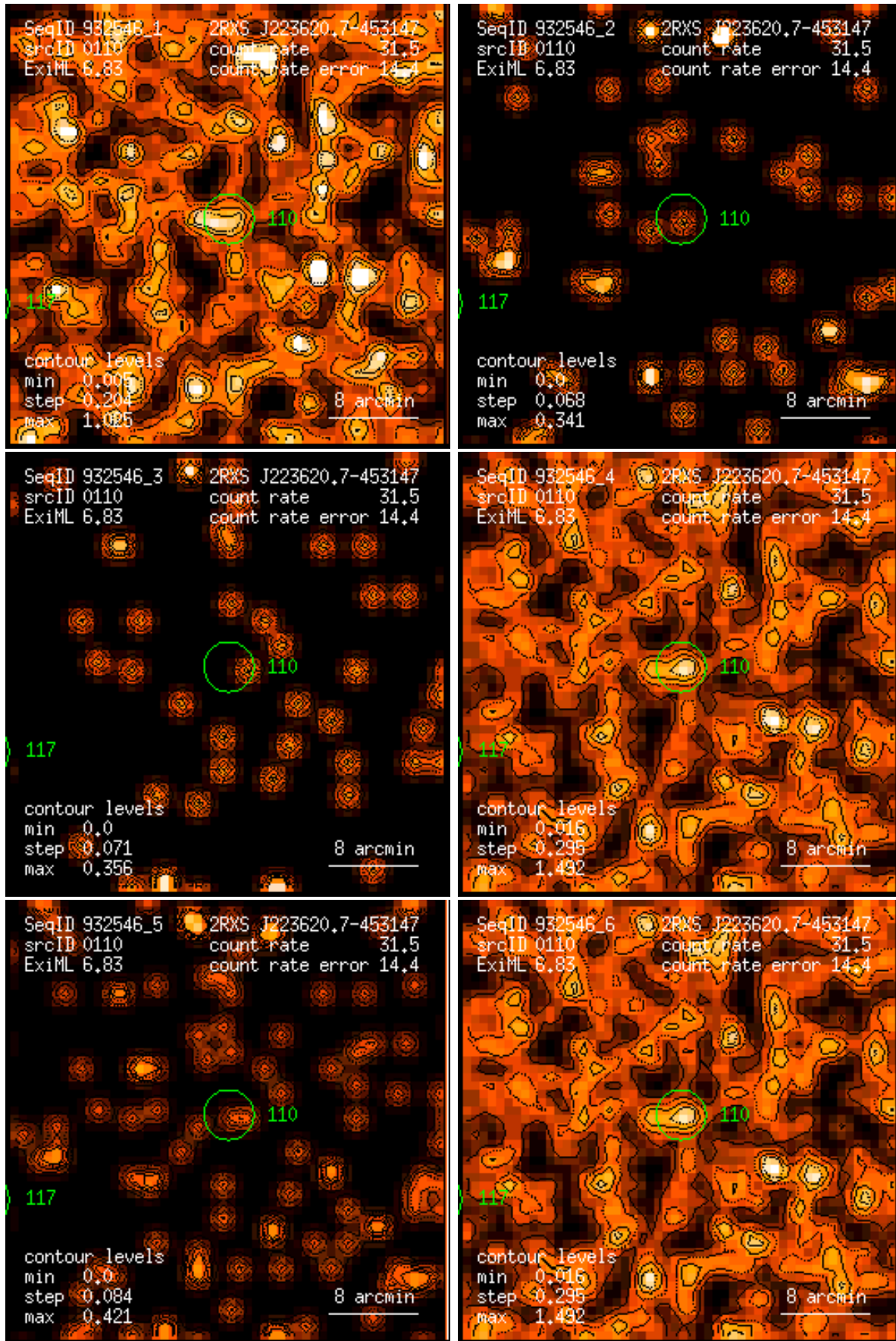
Figure 110: RASS 932546: detection 0110: band rate images, Gaussian filter: (1) PSPC channels 11 – 41, (2) 52 – 90, (3) 91 – 201, (4) 11 – 235, (5) 52 – 201, (6) 11 – 201. Broad band rates in counts/ks. Band rate contour levels in counts/ks/arcmin 2 .
