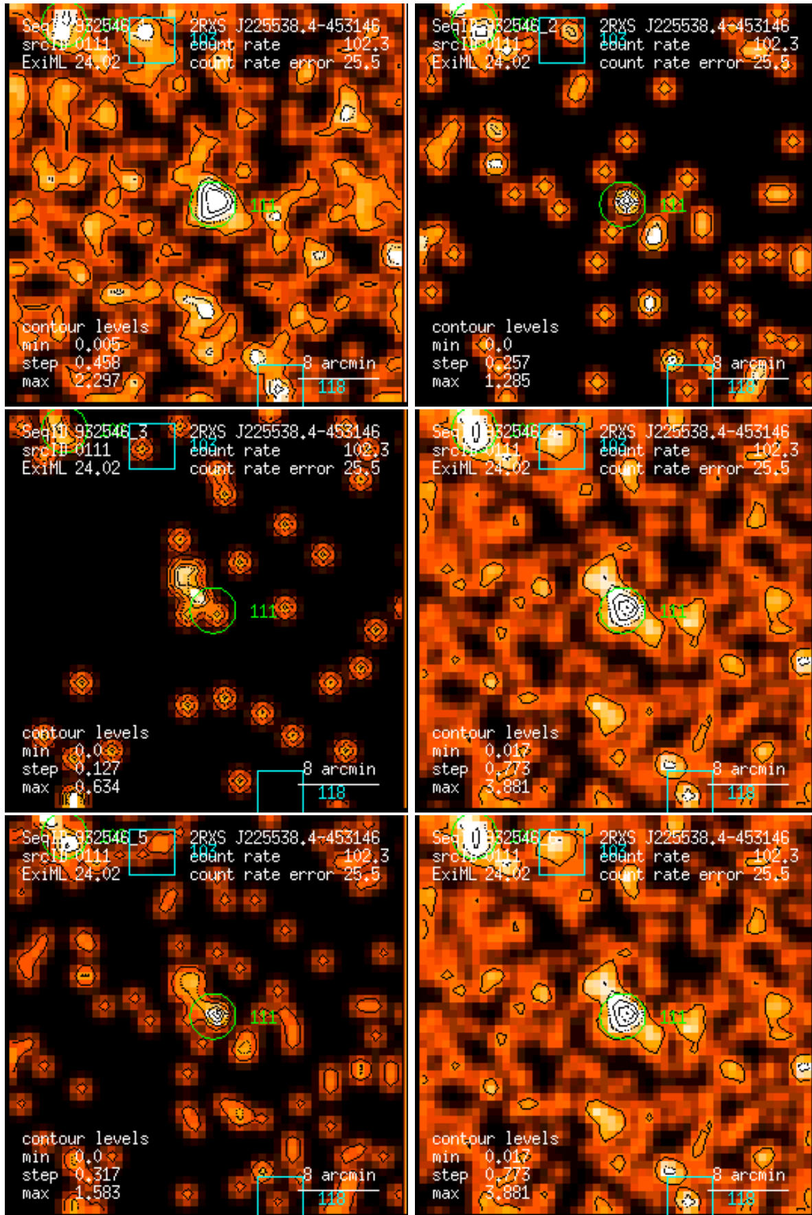
Figure 111: RASS 932546: detection 0111: band rate images, Gaussian filter: (1) PSPC channels 11 – 41, (2) 52 – 90, (3) 91 – 201, (4) 11 – 235, (5) 52 – 201, (6) 11 – 201. Broad band rates in counts/ks. Band rate contour levels in counts/ks/arcmin 2 .
