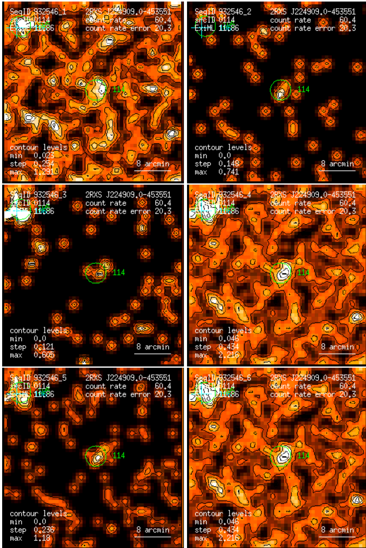
Figure 114: RASS 932546: detection 0114: band rate images, Gaussian filter: (1) PSPC channels 11 – 41, (2) 52 – 90, (3) 91 – 201, (4) 11 – 235, (5) 52 – 201, (6) 11 – 201. Broad band rates in counts/ks. Band rate contour levels in counts/ks/arcmin 2 .
