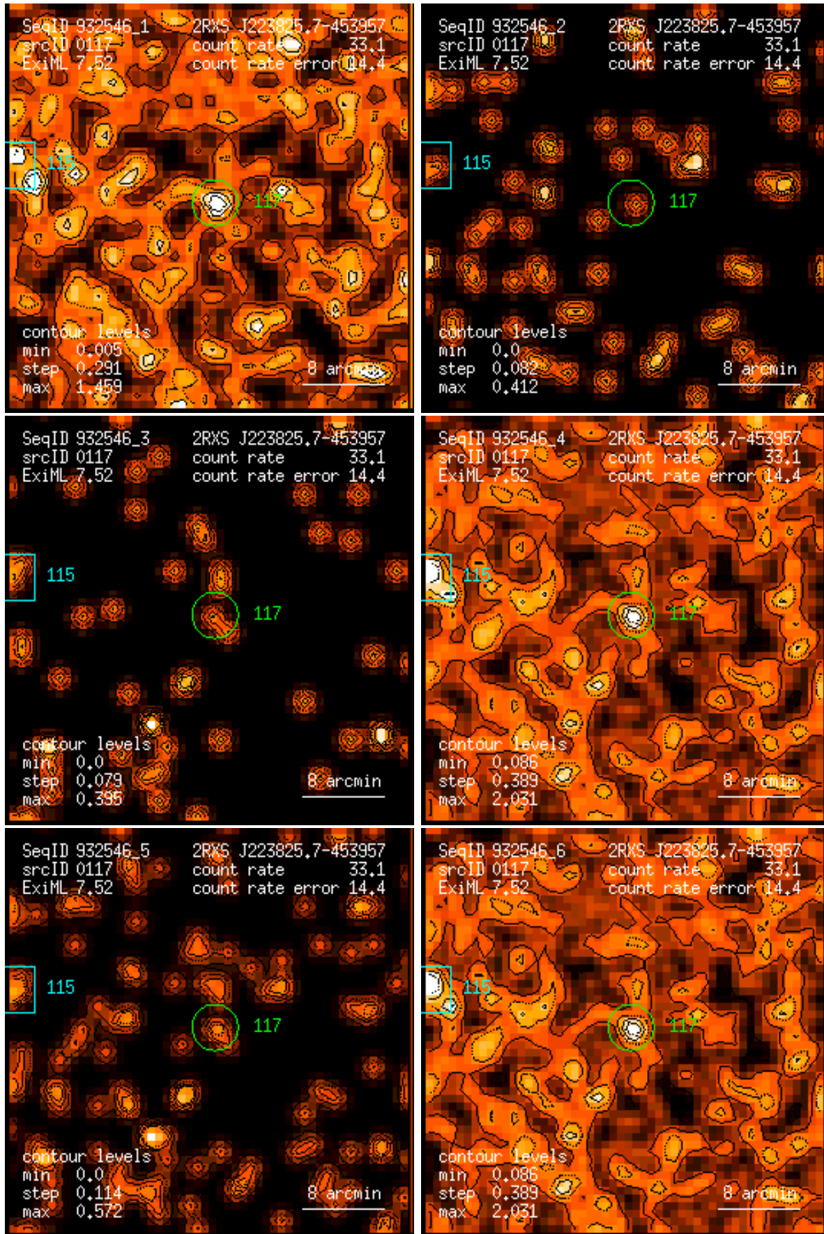
Figure 117: RASS 932546: detection 0117: band rate images, Gaussian filter: (1) PSPC channels 11 – 41, (2) 52 – 90, (3) 91 – 201, (4) 11 – 235, (5) 52 – 201, (6) 11 – 201. Broad band rates in counts/ks. Band rate contour levels in counts/ks/arcmin 2 .
