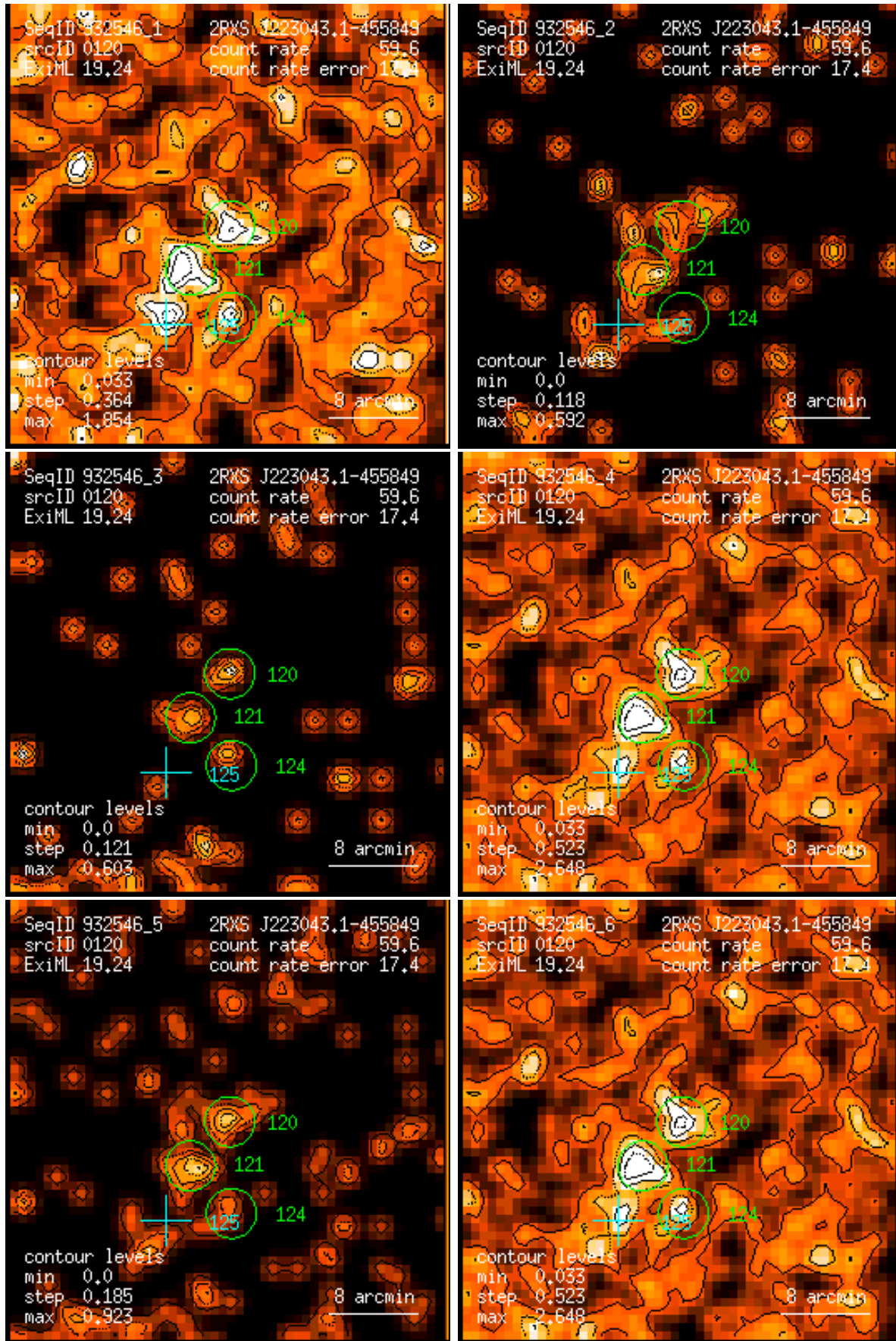
Figure 120: RASS 932546: detection 0120: band rate images, Gaussian filter: (1) PSPC channels 11 – 41, (2) 52 – 90, (3) 91 – 201, (4) 11 – 235, (5) 52 – 201, (6) 11 – 201. Broad band rates in counts/ks. Band rate contour levels in counts/ks/arcmin 2 .
