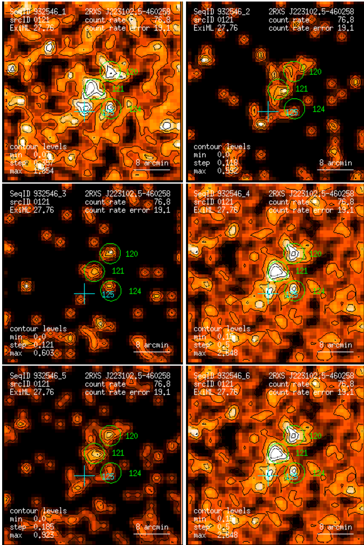
Figure 121: RASS 932546: detection 0121: band rate images, Gaussian filter: (1) PSPC channels 11 – 41, (2) 52 – 90, (3) 91 – 201, (4) 11 – 235, (5) 52 – 201, (6) 11 – 201. Broad band rates in counts/ks. Band rate contour levels in counts/ks/arcmin 2 .
