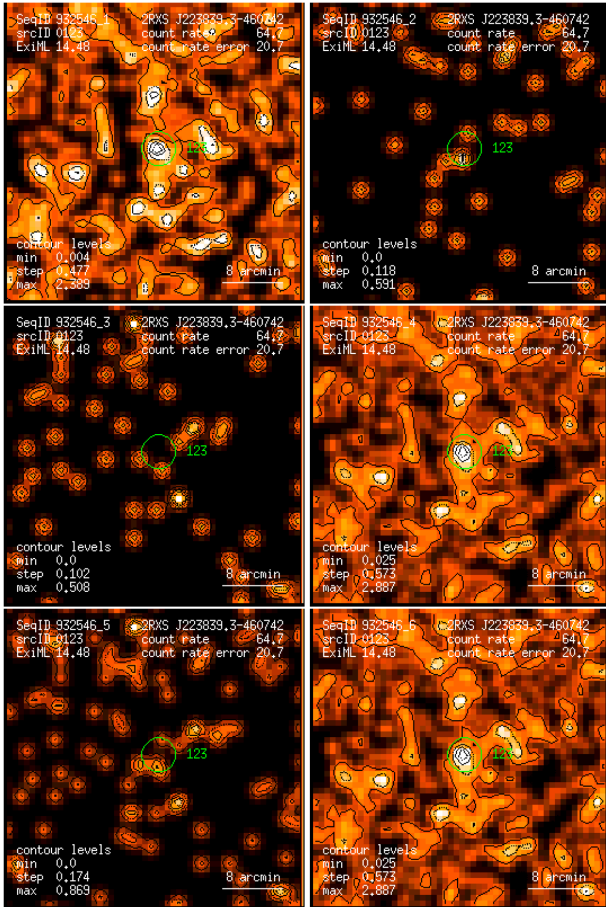
Figure 123: RASS 932546: detection 0123: band rate images, Gaussian filter: (1) PSPC channels 11 – 41, (2) 52 – 90, (3) 91 – 201, (4) 11 – 235, (5) 52 – 201, (6) 11 – 201. Broad band rates in counts/ks. Band rate contour levels in counts/ks/arcmin 2 .
