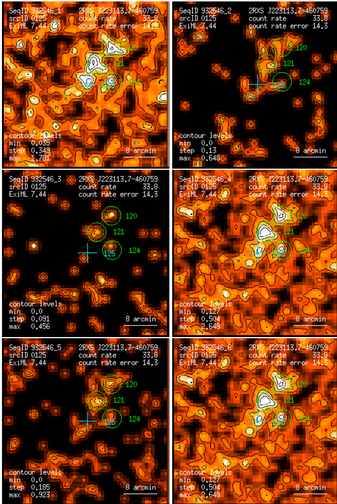
Figure 125: RASS 932546: detection 0125: band rate images, Gaussian filter: (1) PSPC channels 11 – 41, (2) 52 – 90, (3) 91 – 201, (4) 11 – 235, (5) 52 – 201, (6) 11 – 201. Broad band rates in counts/ks. Band rate contour levels in counts/ks/arcmin 2 .
