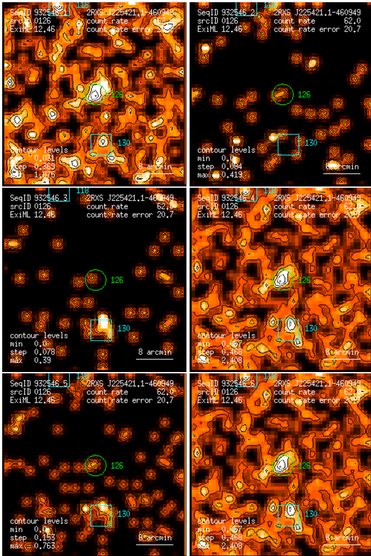
Figure 126: RASS 932546: detection 0126: band rate images, Gaussian filter: (1) PSPC channels 11 – 41, (2) 52 – 90, (3) 91 – 201, (4) 11 – 235, (5) 52 – 201, (6) 11 – 201. Broad band rates in counts/ks. Band rate contour levels in counts/ks/arcmin 2 .
