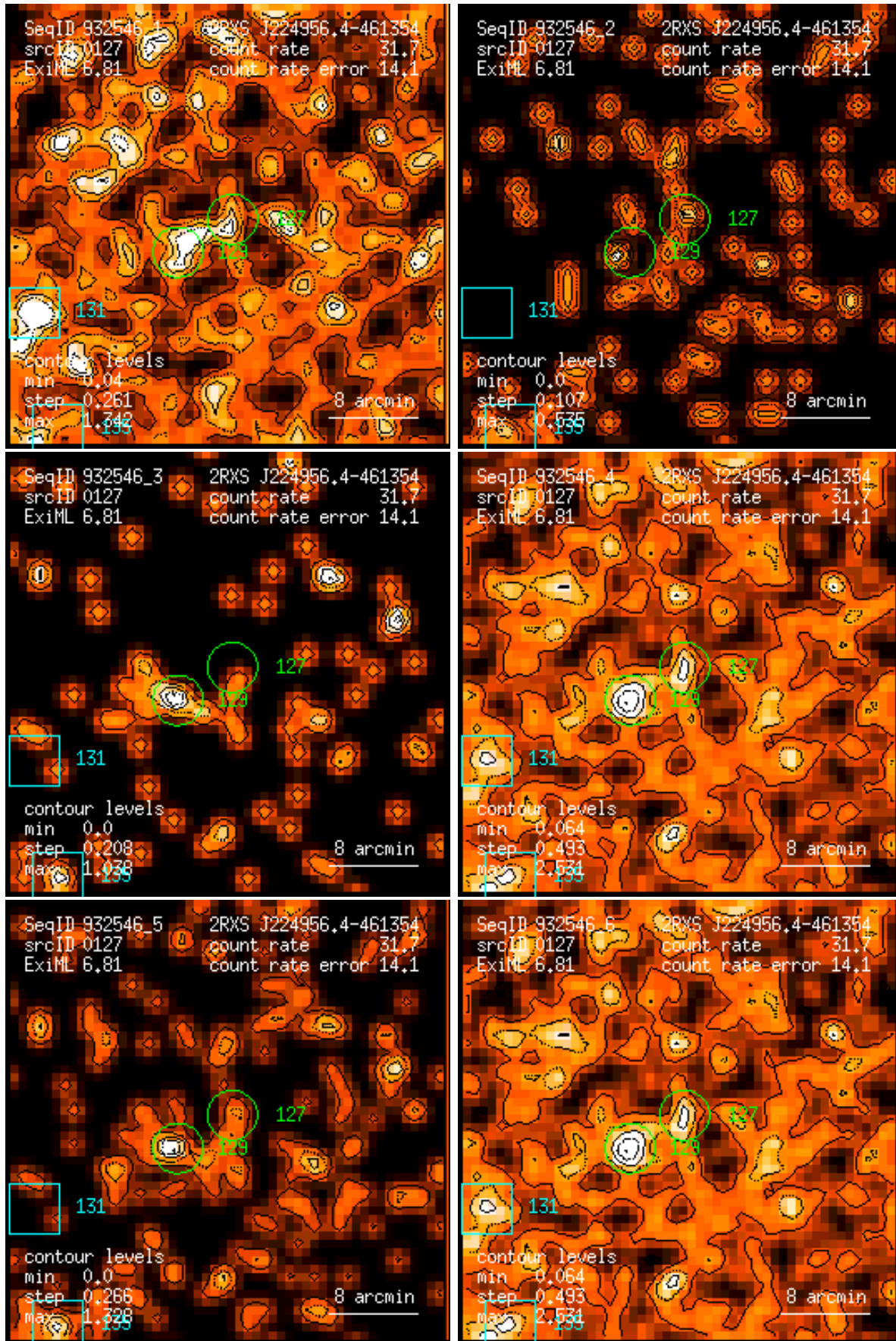
Figure 127: RASS 932546: detection 0127: band rate images, Gaussian filter: (1) PSPC channels 11 – 41, (2) 52 – 90, (3) 91 – 201, (4) 11 – 235, (5) 52 – 201, (6) 11 – 201. Broad band rates in counts/ks. Band rate contour levels in counts/ks/arcmin 2 .
