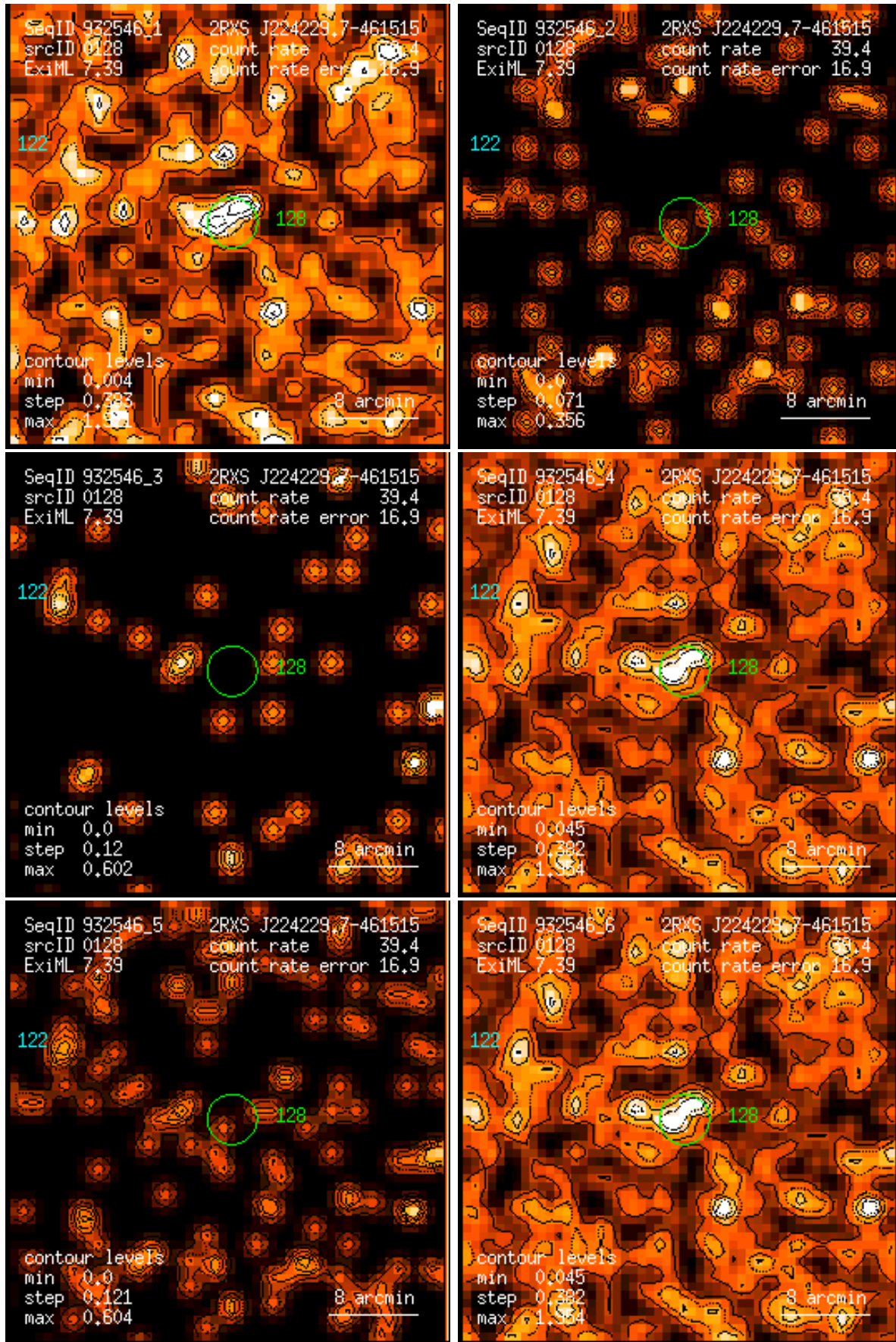
Figure 128: RASS 932546: detection 0128: band rate images, Gaussian filter: (1) PSPC channels 11 – 41, (2) 52 – 90, (3) 91 – 201, (4) 11 – 235, (5) 52 – 201, (6) 11 – 201. Broad band rates in counts/ks. Band rate contour levels in counts/ks/arcmin 2 .
