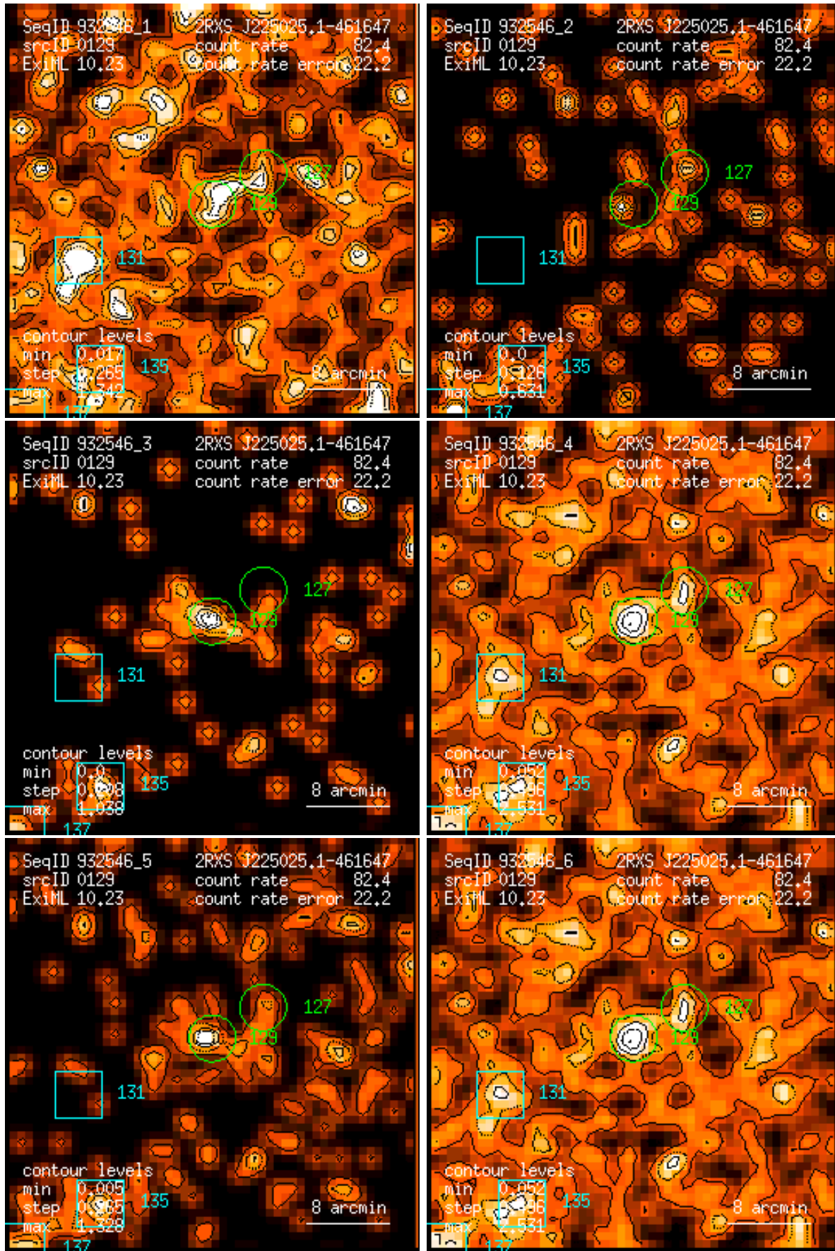
Figure 129: RASS 932546: detection 0129: band rate images, Gaussian filter: (1) PSPC channels 11 – 41, (2) 52 – 90, (3) 91 – 201, (4) 11 – 235, (5) 52 – 201, (6) 11 – 201. Broad band rates in counts/ks. Band rate contour levels in counts/ks/arcmin 2 .
