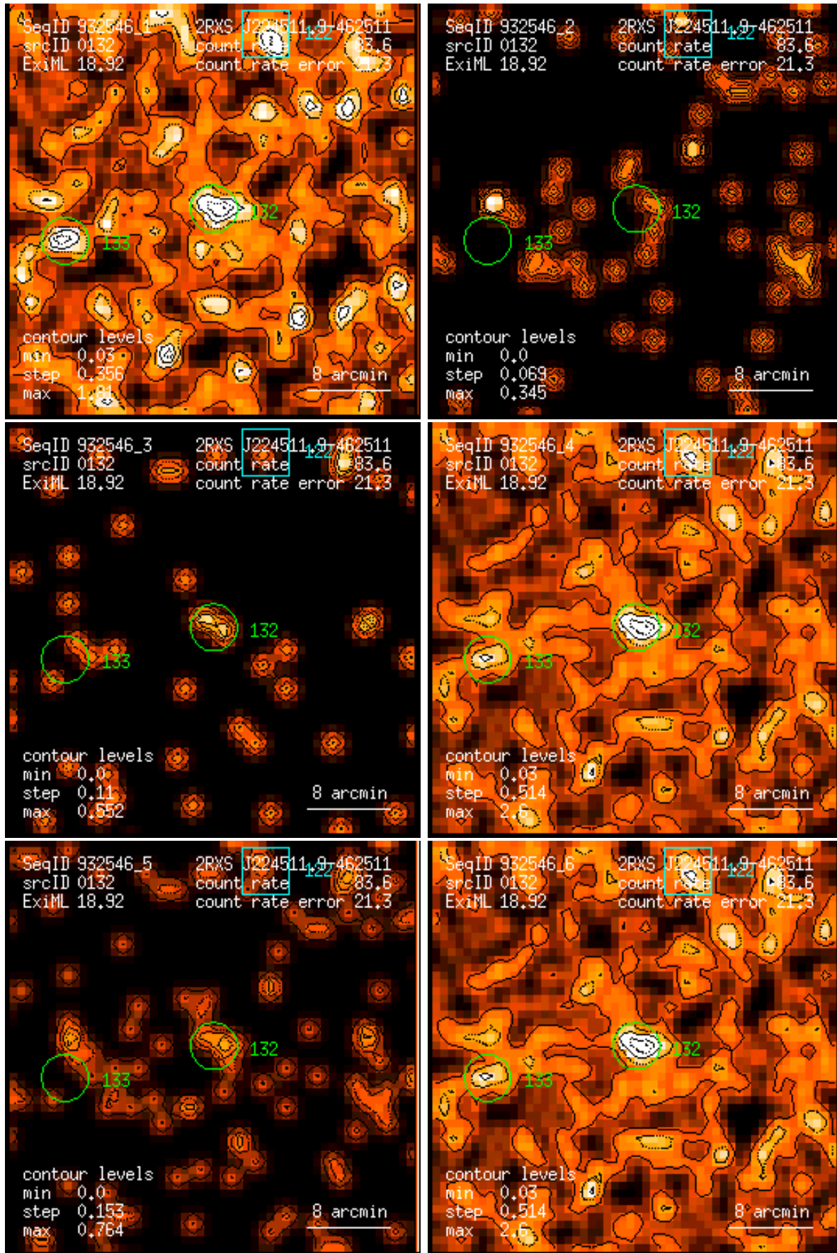
Figure 132: RASS 932546: detection 0132: band rate images, Gaussian filter: (1) PSPC channels 11 – 41, (2) 52 – 90, (3) 91 – 201, (4) 11 – 235, (5) 52 – 201, (6) 11 – 201. Broad band rates in counts/ks. Band rate contour levels in counts/ks/arcmin 2 .
