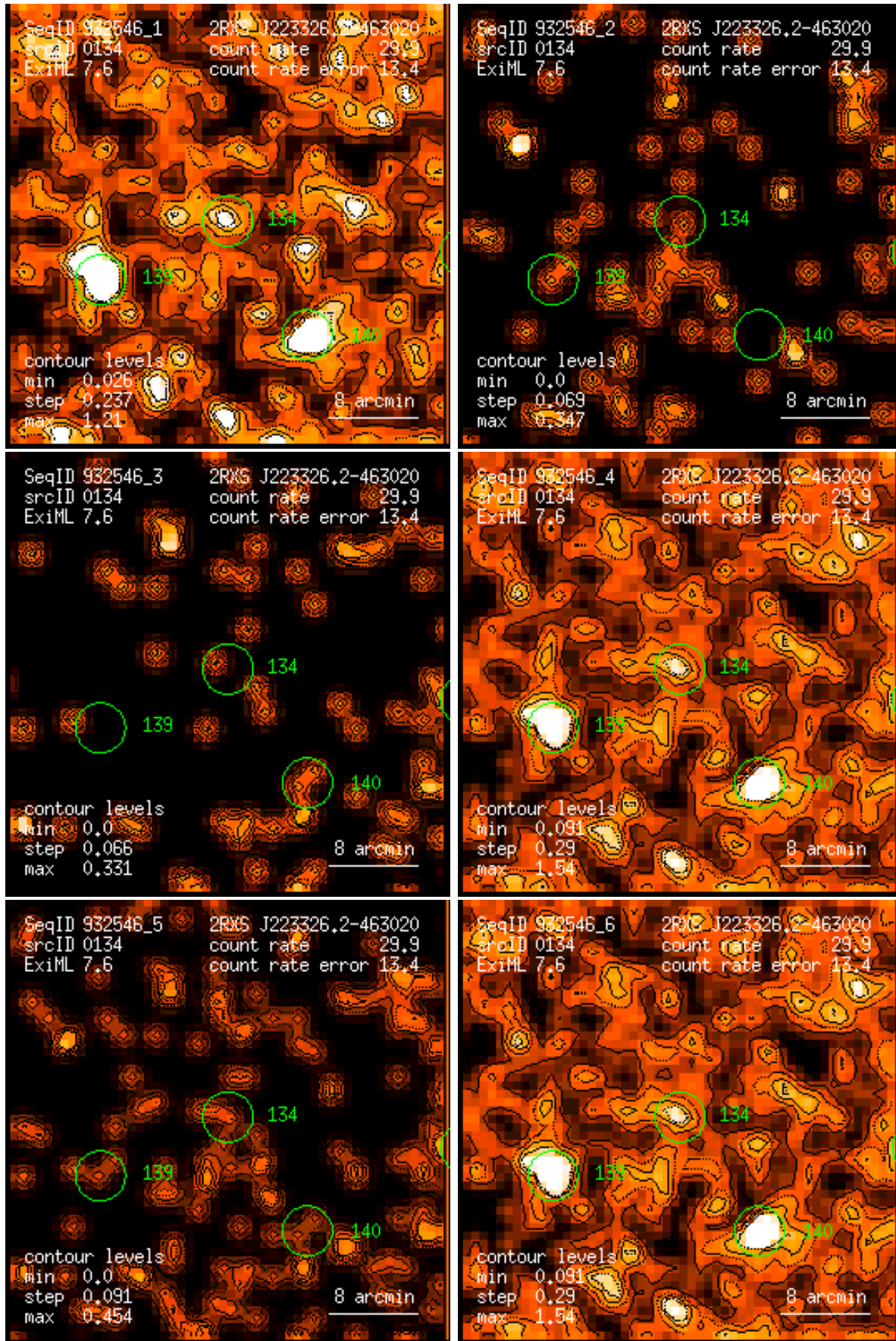
Figure 134: RASS 932546: detection 0134: band rate images, Gaussian filter: (1) PSPC channels 11 – 41, (2) 52 – 90, (3) 91 – 201, (4) 11 – 235, (5) 52 – 201, (6) 11 – 201. Broad band rates in counts/ks. Band rate contour levels in counts/ks/arcmin 2 .
