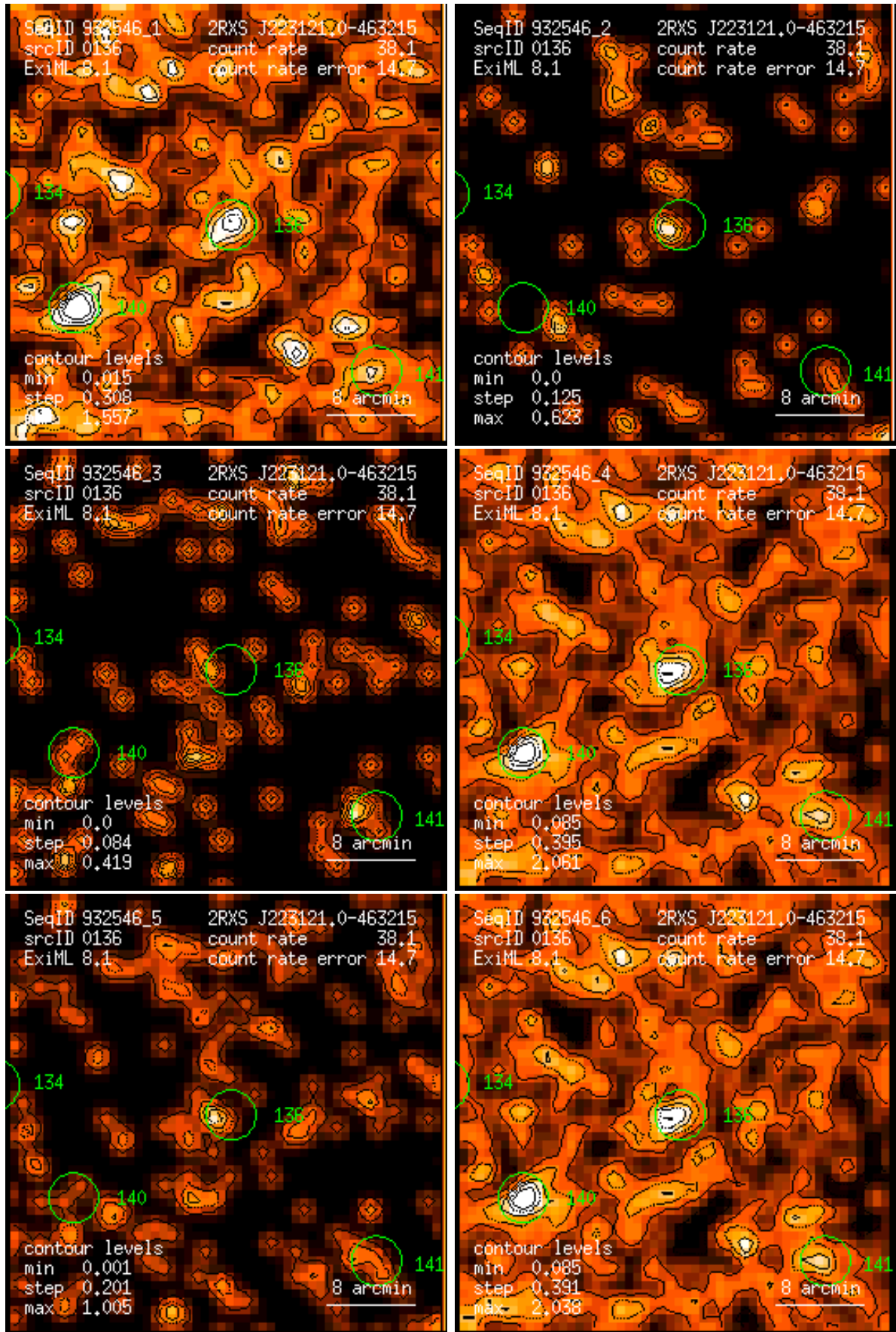
Figure 136: RASS 932546: detection 0136: band rate images, Gaussian filter: (1) PSPC channels 11 – 41, (2) 52 – 90, (3) 91 – 201, (4) 11 – 235, (5) 52 – 201, (6) 11 – 201. Broad band rates in counts/ks. Band rate contour levels in counts/ks/arcmin 2 .
