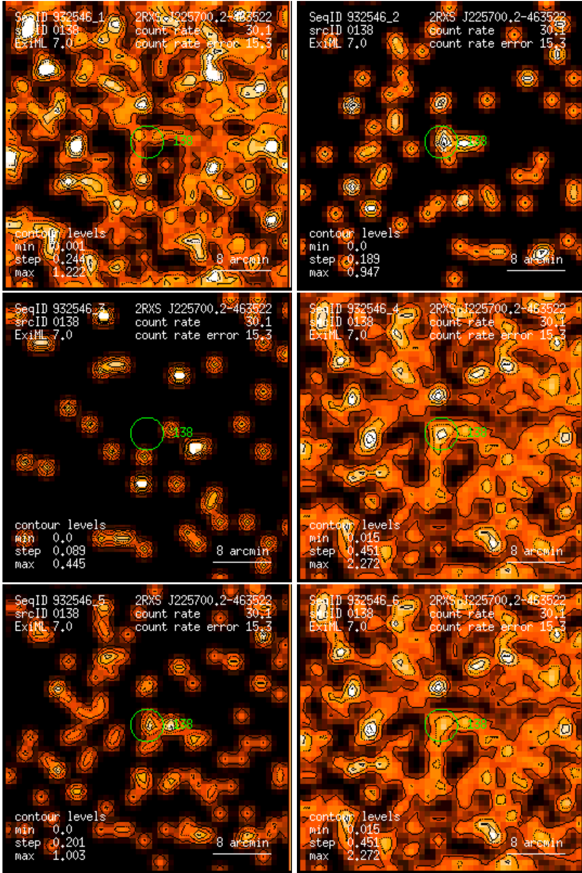
Figure 138: RASS 932546: detection 0138: band rate images, Gaussian filter: (1) PSPC channels 11 – 41, (2) 52 – 90, (3) 91 – 201, (4) 11 – 235, (5) 52 – 201, (6) 11 – 201. Broad band rates in counts/ks. Band rate contour levels in counts/ks/arcmin 2 .
