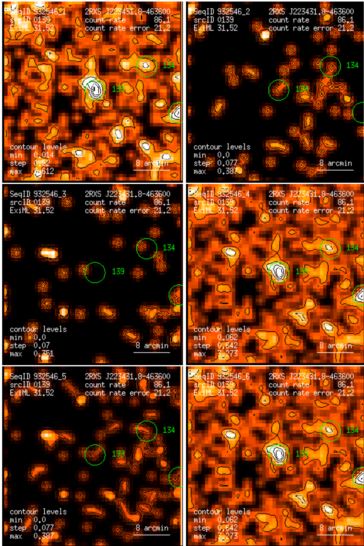
Figure 139: RASS 932546: detection 0139: band rate images, Gaussian filter: (1) PSPC channels 11 – 41, (2) 52 – 90, (3) 91 – 201, (4) 11 – 235, (5) 52 – 201, (6) 11 – 201. Broad band rates in counts/ks. Band rate contour levels in counts/ks/arcmin 2 .
