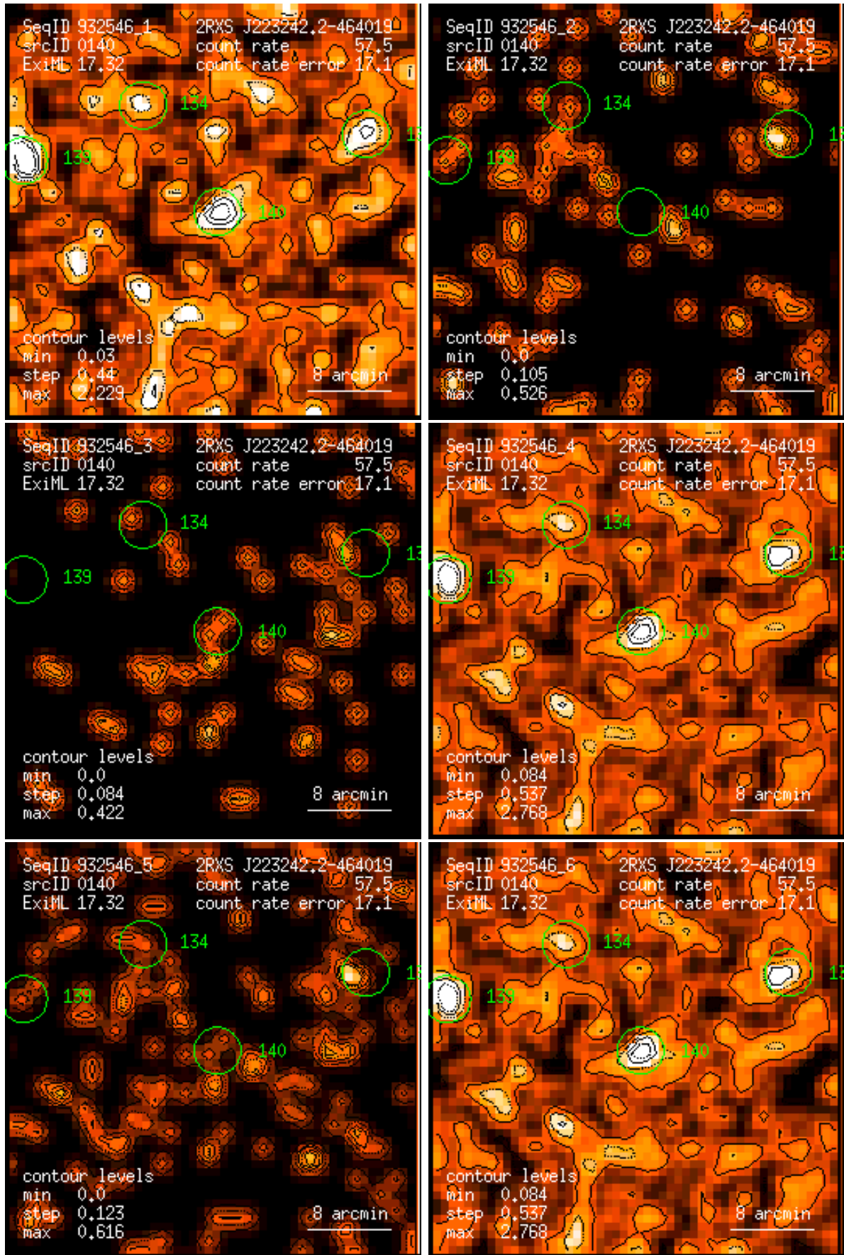
Figure 140: RASS 932546: detection 0140: band rate images, Gaussian filter: (1) PSPC channels 11 – 41, (2) 52 – 90, (3) 91 – 201, (4) 11 – 235, (5) 52 – 201, (6) 11 – 201. Broad band rates in counts/ks. Band rate contour levels in counts/ks/arcmin 2 .
