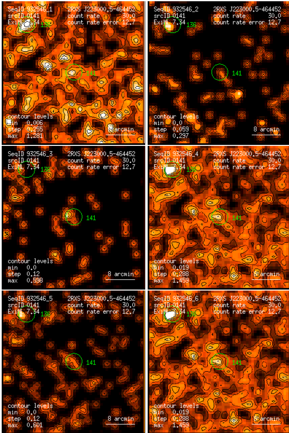
Figure 141: RASS 932546: detection 0141: band rate images, Gaussian filter: (1) PSPC channels 11 – 41, (2) 52 – 90, (3) 91 – 201, (4) 11 – 235, (5) 52 – 201, (6) 11 – 201. Broad band rates in counts/ks. Band rate contour levels in counts/ks/arcmin 2 .
