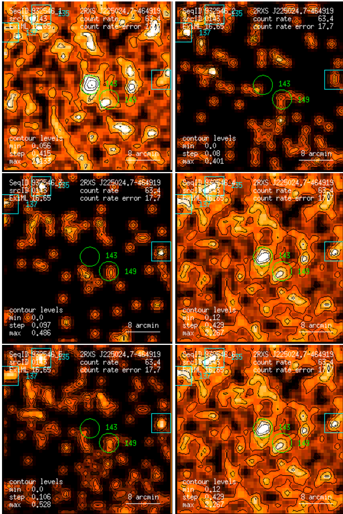
Figure 143: RASS 932546: detection 0143: band rate images, Gaussian filter: (1) PSPC channels 11 – 41, (2) 52 – 90, (3) 91 – 201, (4) 11 – 235, (5) 52 – 201, (6) 11 – 201. Broad band rates in counts/ks. Band rate contour levels in counts/ks/arcmin 2 .
