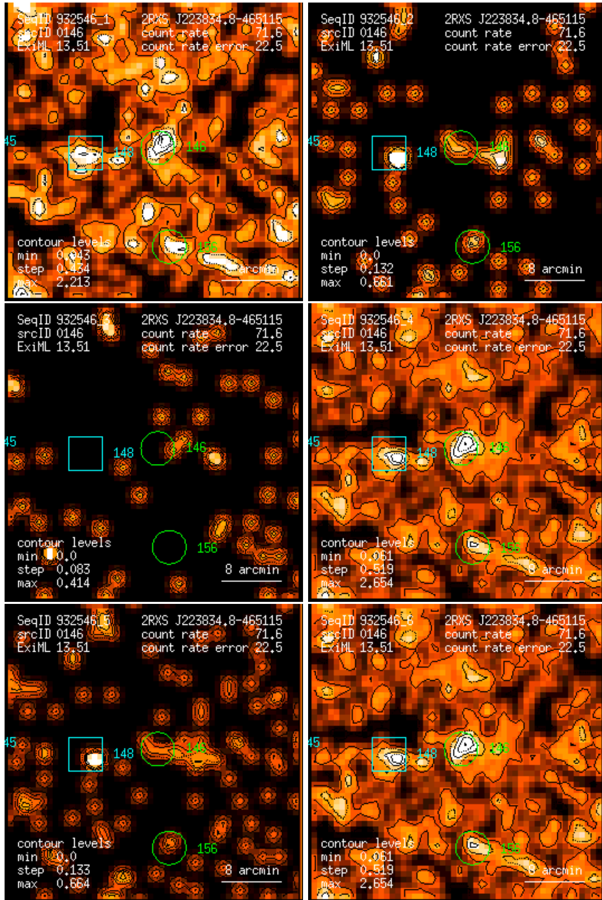
Figure 146: RASS 932546: detection 0146: band rate images, Gaussian filter: (1) PSPC channels 11 – 41, (2) 52 – 90, (3) 91 – 201, (4) 11 – 235, (5) 52 – 201, (6) 11 – 201. Broad band rates in counts/ks. Band rate contour levels in counts/ks/arcmin 2 .
