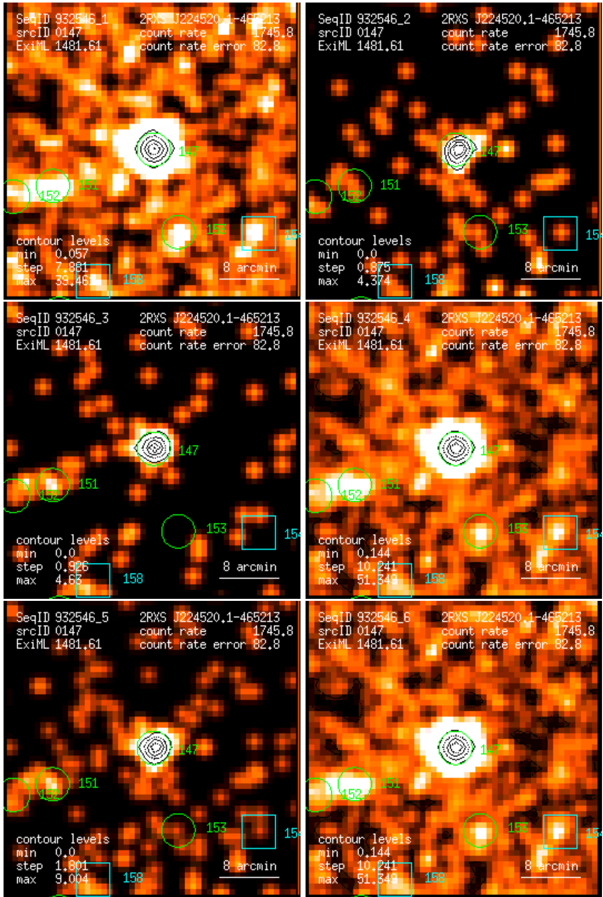
Figure 147: RASS 932546: detection 0147: band rate images, Gaussian filter: (1) PSPC channels 11 – 41, (2) 52 – 90, (3) 91 – 201, (4) 11 – 235, (5) 52 – 201, (6) 11 – 201. Broad band rates in counts/ks. Band rate contour levels in counts/ks/arcmin 2 .
