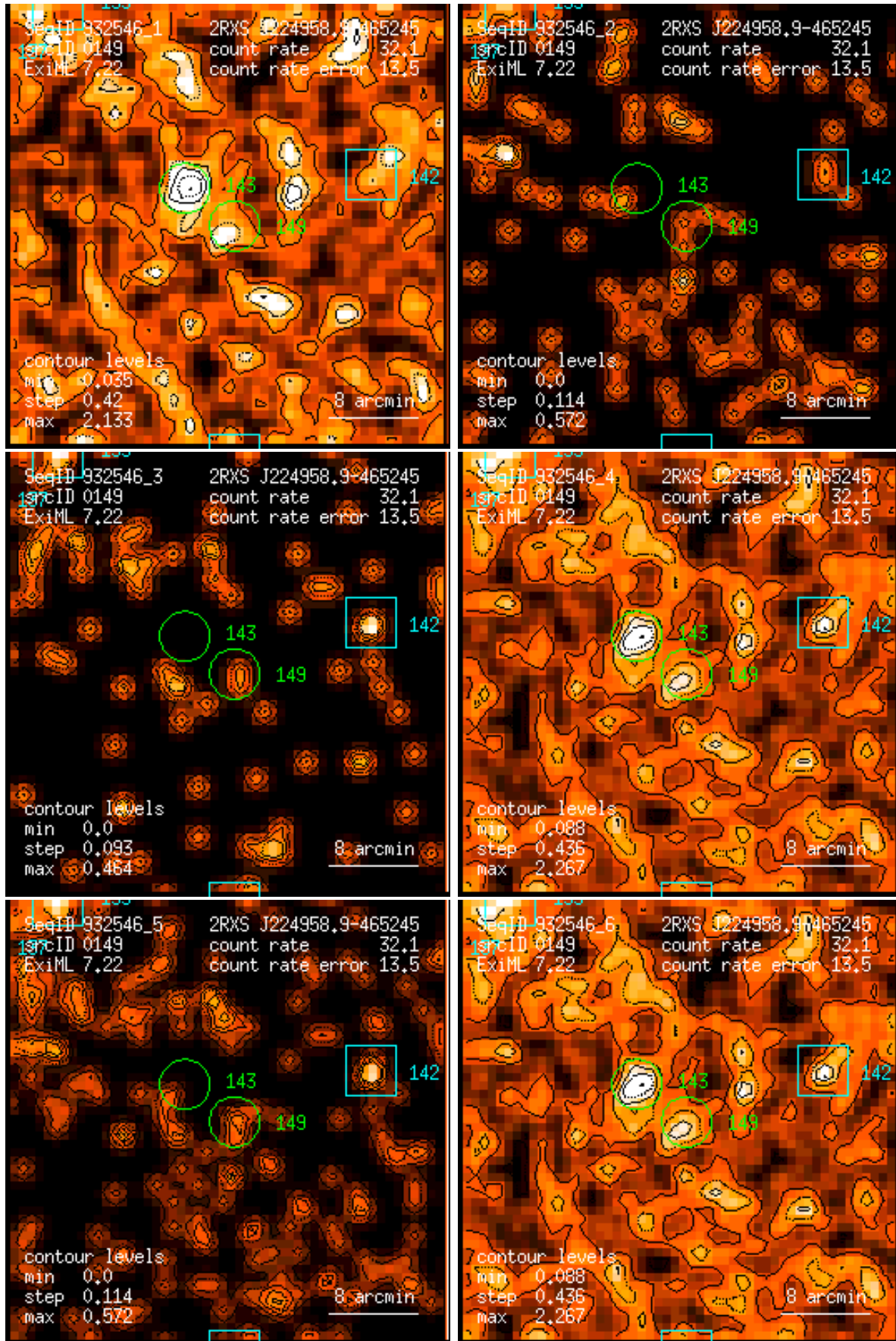
Figure 149: RASS 932546: detection 0149: band rate images, Gaussian filter: (1) PSPC channels 11 – 41, (2) 52 – 90, (3) 91 – 201, (4) 11 – 235, (5) 52 – 201, (6) 11 – 201. Broad band rates in counts/ks. Band rate contour levels in counts/ks/arcmin 2 .
