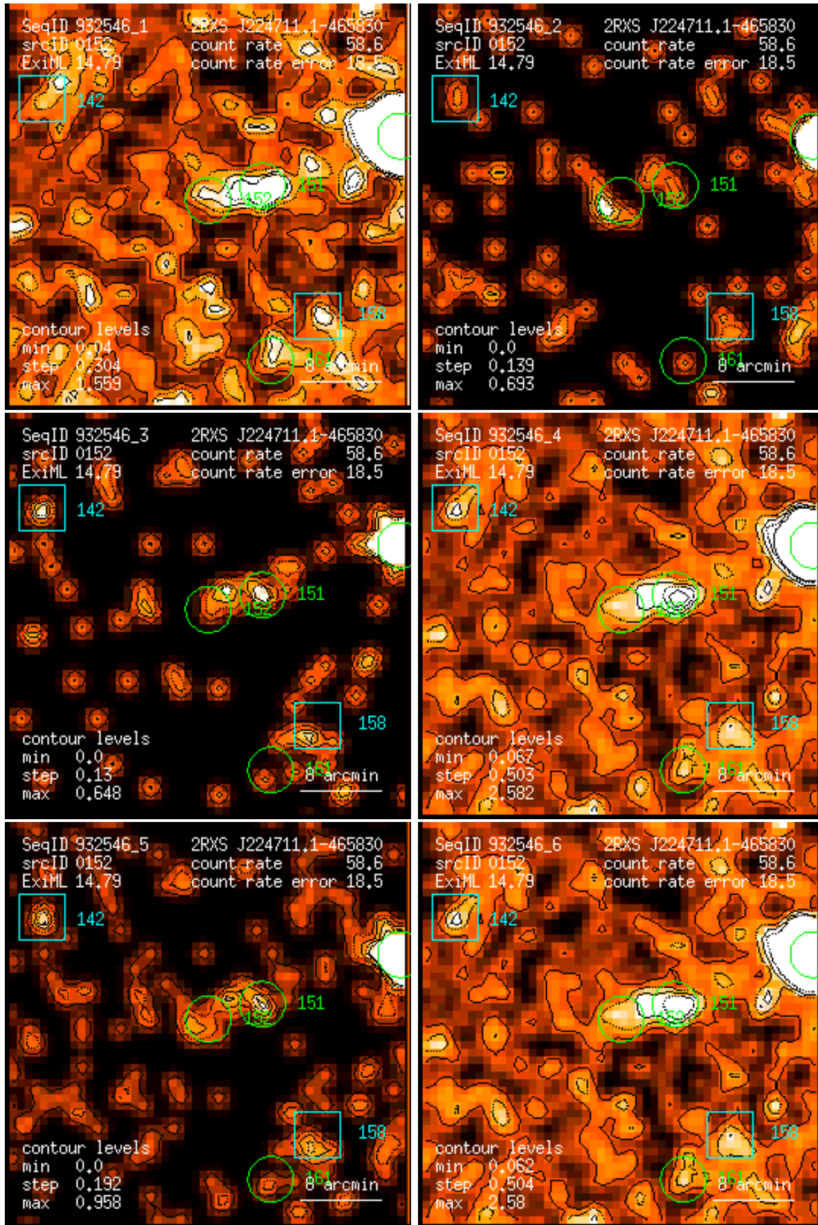
Figure 152: RASS 932546: detection 0152: band rate images, Gaussian filter: (1) PSPC channels 11 – 41, (2) 52 – 90, (3) 91 – 201, (4) 11 – 235, (5) 52 – 201, (6) 11 – 201. Broad band rates in counts/ks. Band rate contour levels in counts/ks/arcmin 2 .
