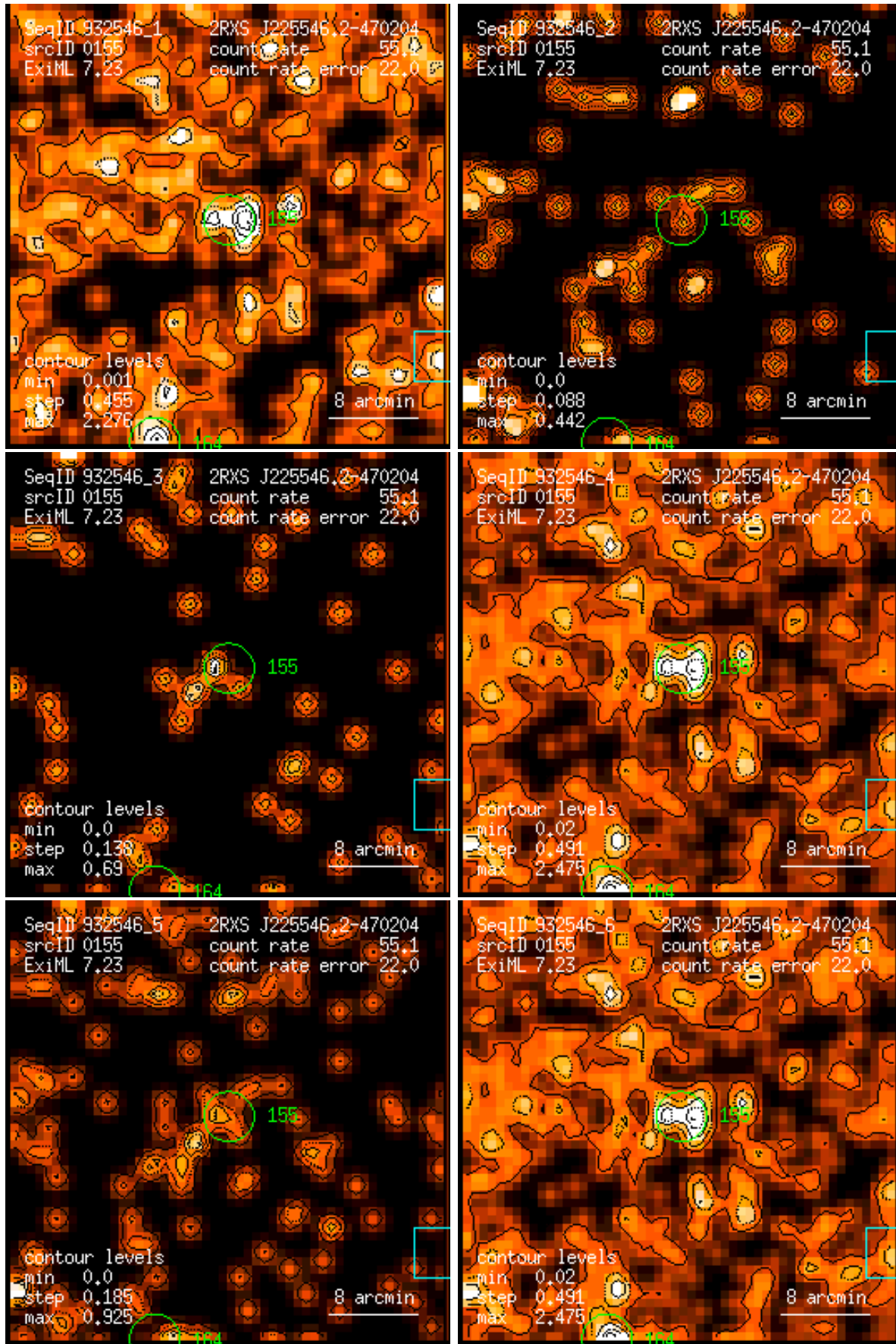
Figure 155: RASS 932546: detection 0155: band rate images, Gaussian filter: (1) PSPC channels 11 – 41, (2) 52 – 90, (3) 91 – 201, (4) 11 – 235, (5) 52 – 201, (6) 11 – 201. Broad band rates in counts/ks. Band rate contour levels in counts/ks/arcmin 2 .
