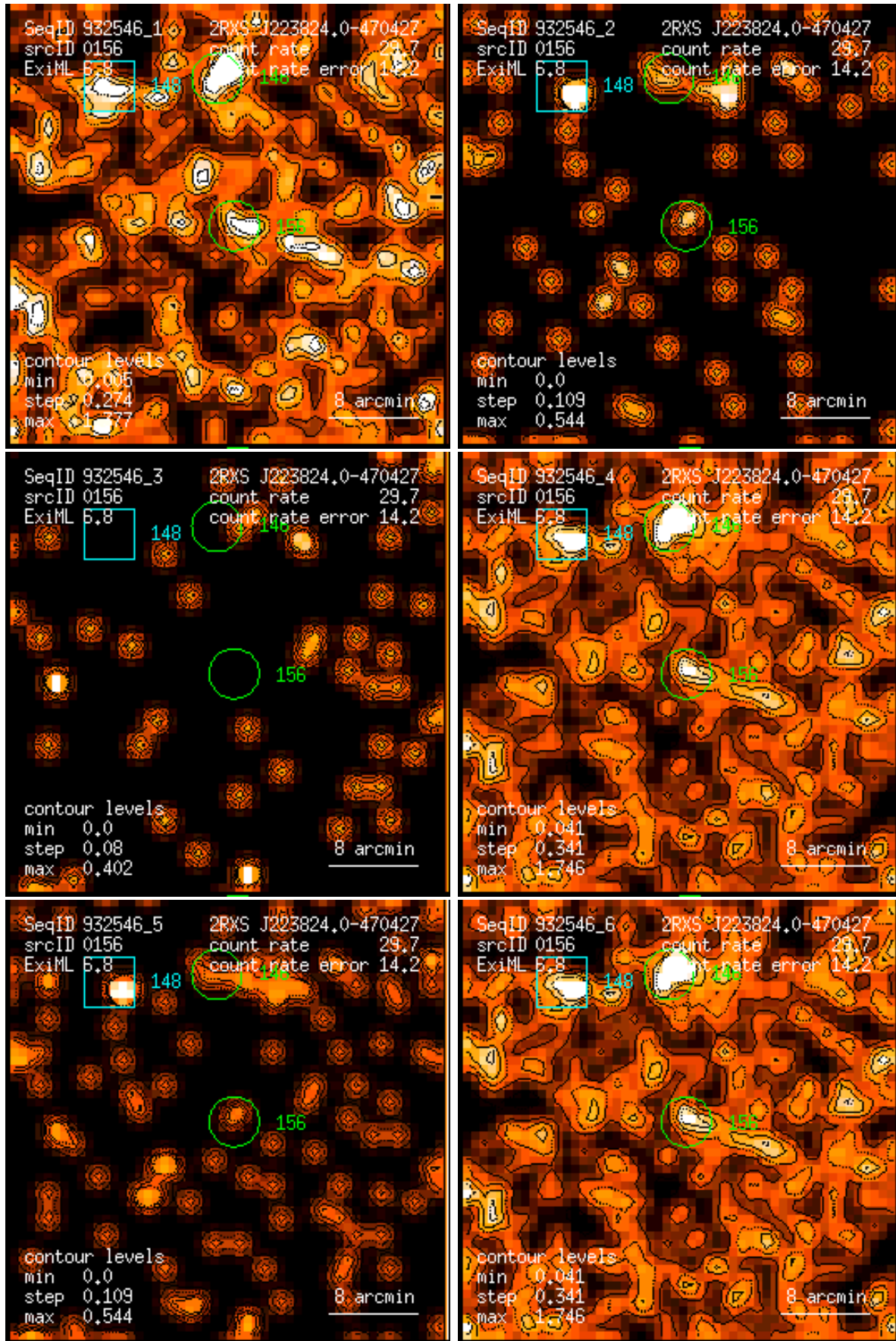
Figure 156: RASS 932546: detection 0156: band rate images, Gaussian filter: (1) PSPC channels 11 – 41, (2) 52 – 90, (3) 91 – 201, (4) 11 – 235, (5) 52 – 201, (6) 11 – 201. Broad band rates in counts/ks. Band rate contour levels in counts/ks/arcmin 2 .
