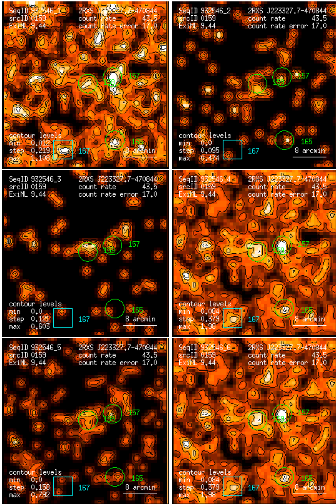
Figure 159: RASS 932546: detection 0159: band rate images, Gaussian filter: (1) PSPC channels 11 – 41, (2) 52 – 90, (3) 91 – 201, (4) 11 – 235, (5) 52 – 201, (6) 11 – 201. Broad band rates in counts/ks. Band rate contour levels in counts/ks/arcmin 2 .
