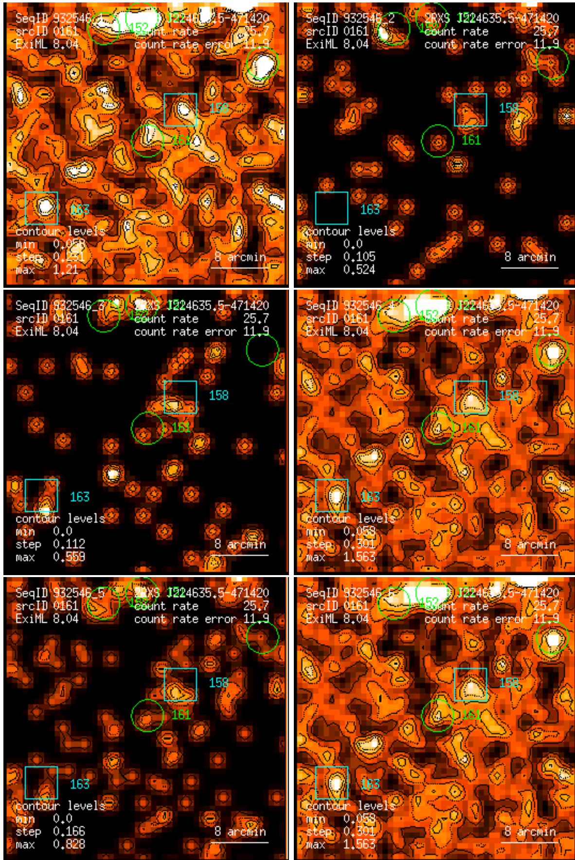
Figure 161: RASS 932546: detection 0161: band rate images, Gaussian filter: (1) PSPC channels 11 – 41, (2) 52 – 90, (3) 91 – 201, (4) 11 – 235, (5) 52 – 201, (6) 11 – 201. Broad band rates in counts/ks. Band rate contour levels in counts/ks/arcmin 2 .
