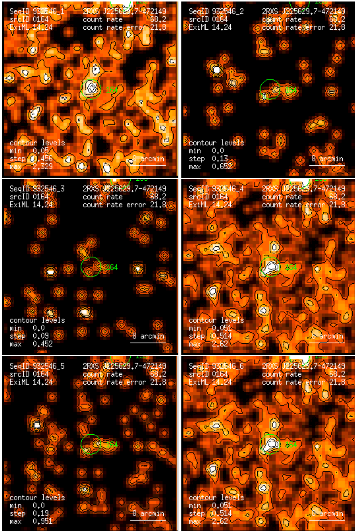
Figure 164: RASS 932546: detection 0164: band rate images, Gaussian filter: (1) PSPC channels 11 – 41, (2) 52 – 90, (3) 91 – 201, (4) 11 – 235, (5) 52 – 201, (6) 11 – 201. Broad band rates in counts/ks. Band rate contour levels in counts/ks/arcmin 2 .
