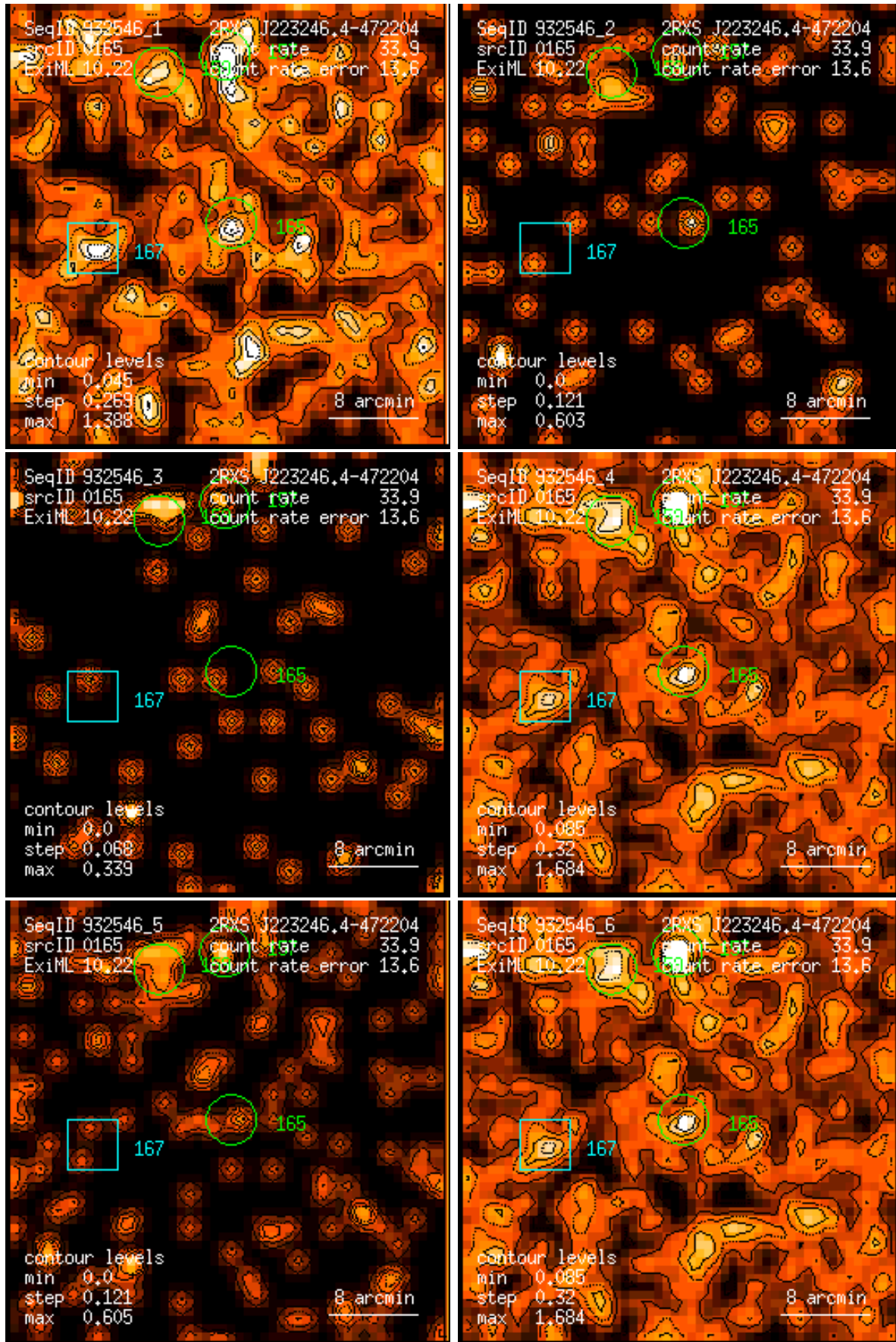
Figure 165: RASS 932546: detection 0165: band rate images, Gaussian filter: (1) PSPC channels 11 – 41, (2) 52 – 90, (3) 91 – 201, (4) 11 – 235, (5) 52 – 201, (6) 11 – 201. Broad band rates in counts/ks. Band rate contour levels in counts/ks/arcmin 2 .
