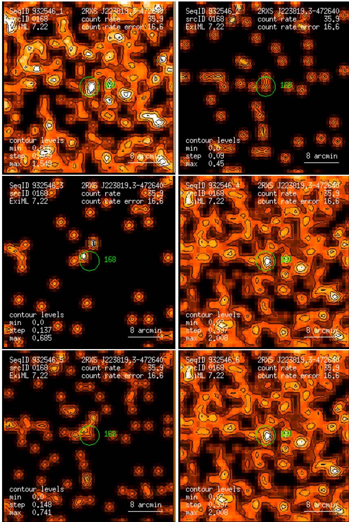
Figure 168: RASS 932546: detection 0168: band rate images, Gaussian filter: (1) PSPC channels 11 – 41, (2) 52 – 90, (3) 91 – 201, (4) 11 – 235, (5) 52 – 201, (6) 11 – 201. Broad band rates in counts/ks. Band rate contour levels in counts/ks/arcmin 2 .
