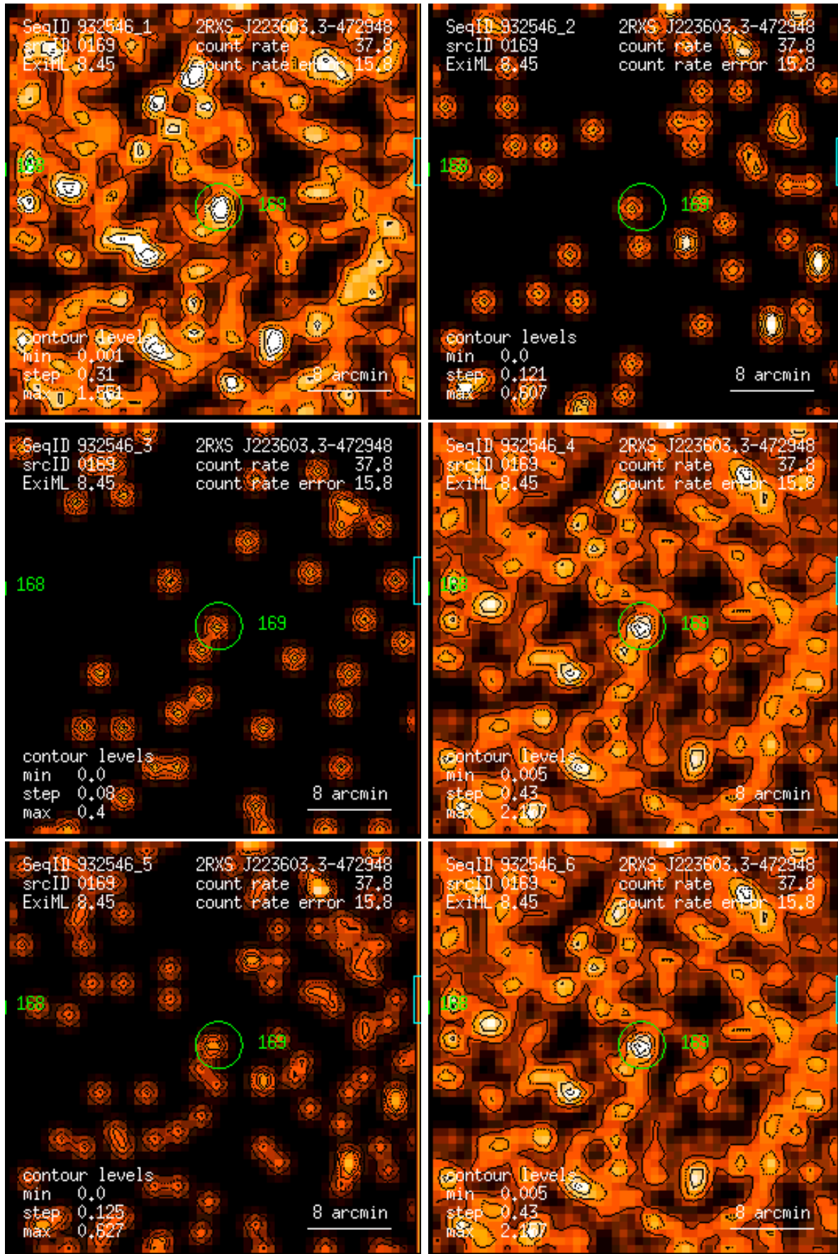
Figure 169: RASS 932546: detection 0169: band rate images, Gaussian filter: (1) PSPC channels 11 – 41, (2) 52 – 90, (3) 91 – 201, (4) 11 – 235, (5) 52 – 201, (6) 11 – 201. Broad band rates in counts/ks. Band rate contour levels in counts/ks/arcmin 2 .
