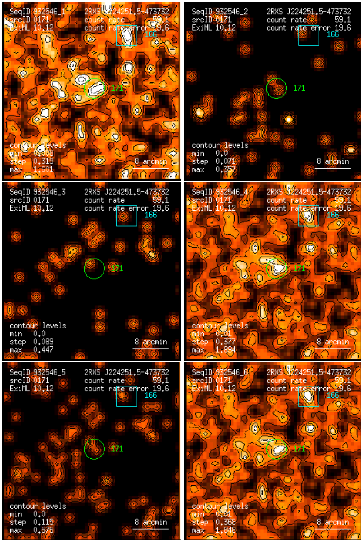
Figure 171: RASS 932546: detection 0171: band rate images, Gaussian filter: (1) PSPC channels 11 – 41, (2) 52 – 90, (3) 91 – 201, (4) 11 – 235, (5) 52 – 201, (6) 11 – 201. Broad band rates in counts/ks. Band rate contour levels in counts/ks/arcmin 2 .
